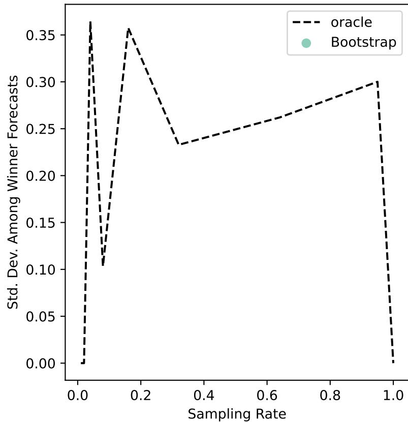
ers-16 Uncertainty
