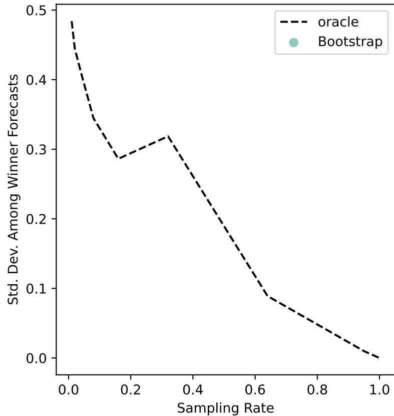
ers-47 Uncertainty
