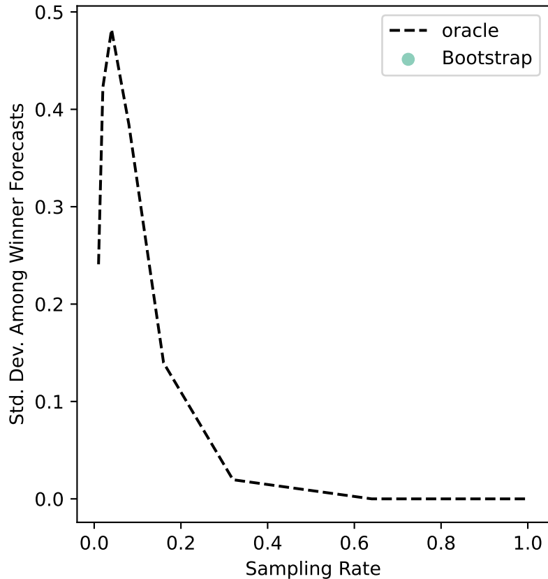
ers-71 Uncertainty
