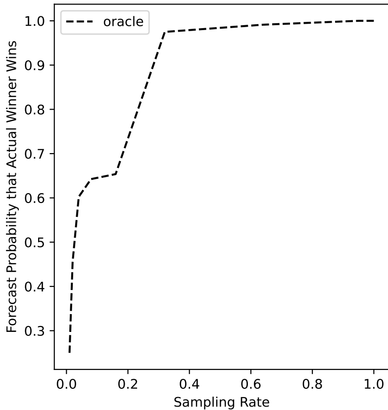
ers-74 Forecast
