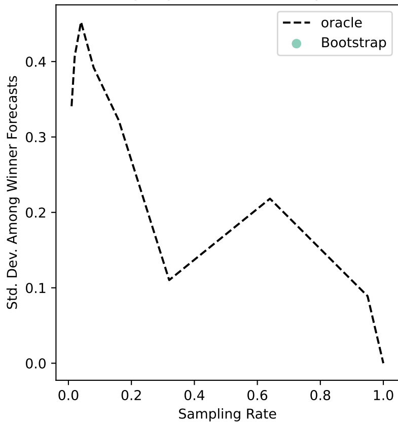
glasgow-01 Uncertainty
