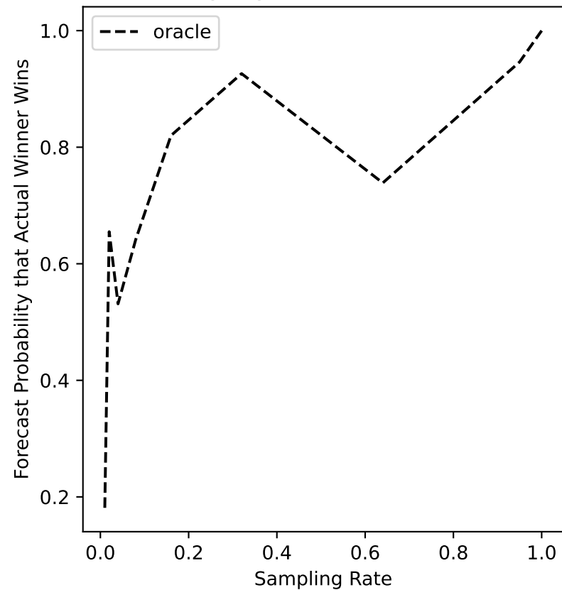
glasgow-01 Forecast
