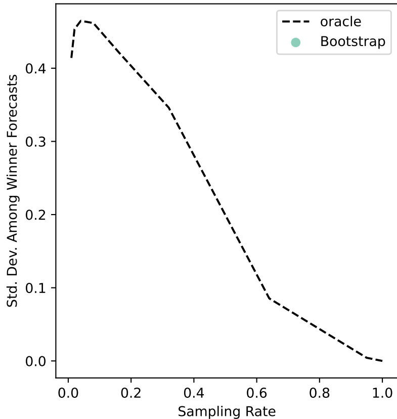
glasgow-05 Uncertainty
