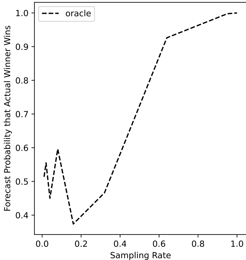
glasgow-05 Forecast
