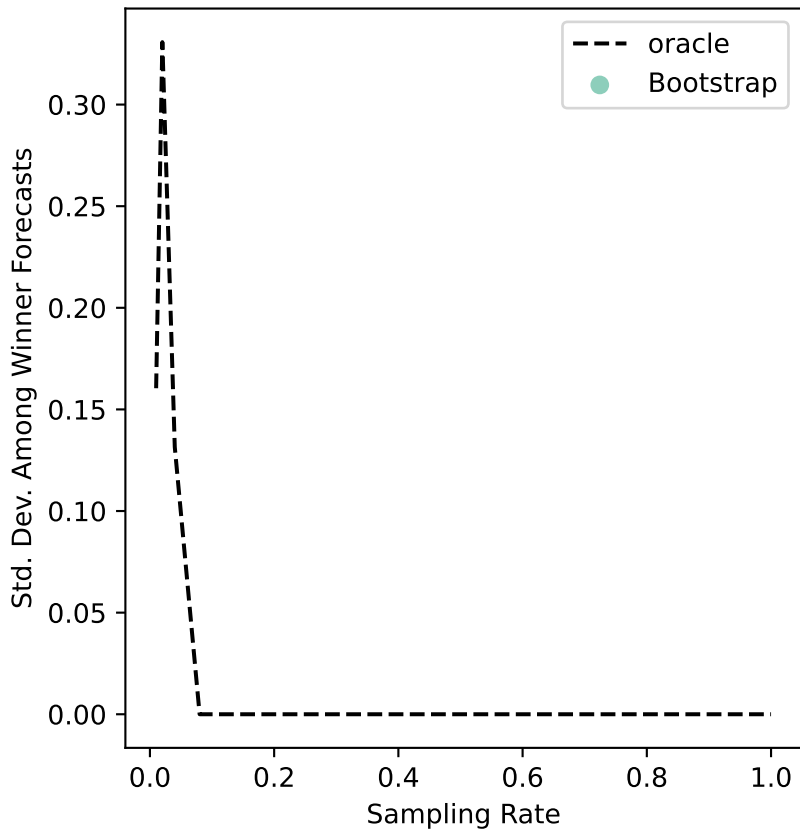
glasgow-06 Uncertainty
