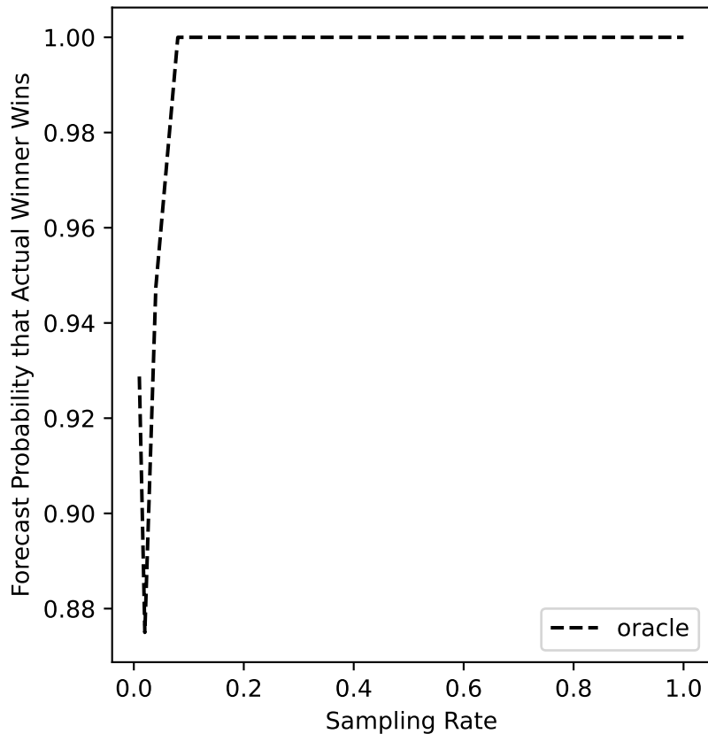
glasgow-06 Forecast
