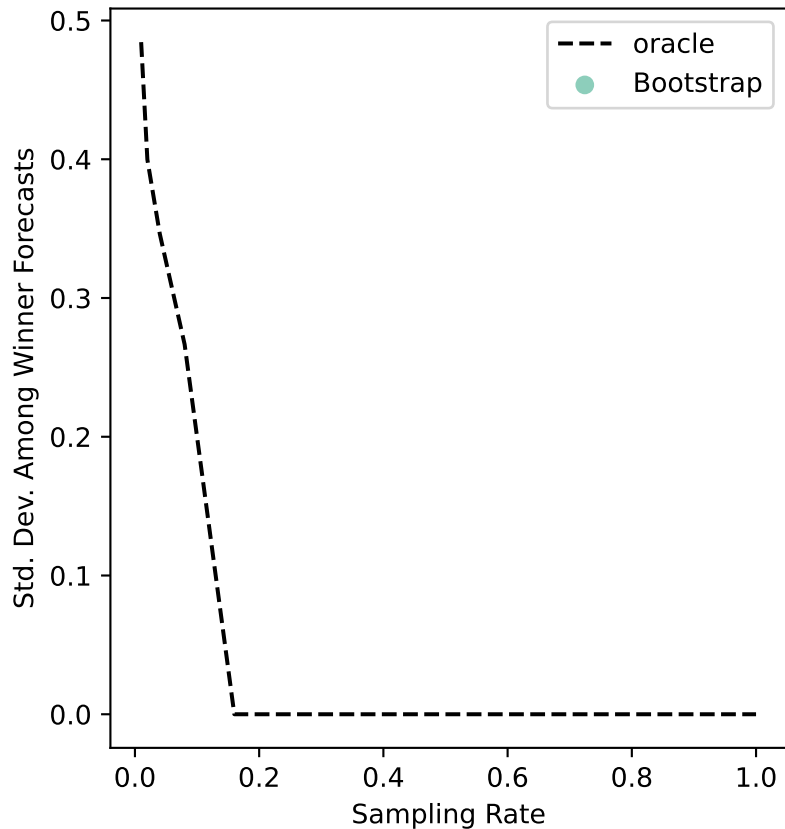
glasgow-13 Uncertainty
