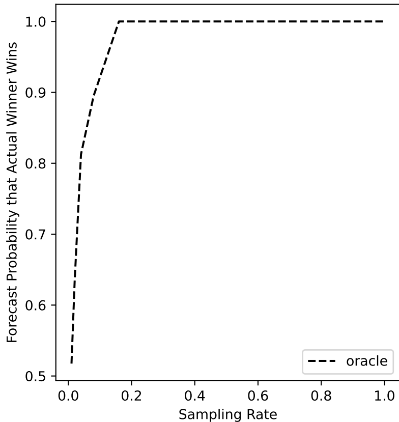
glasgow-13 Forecast
