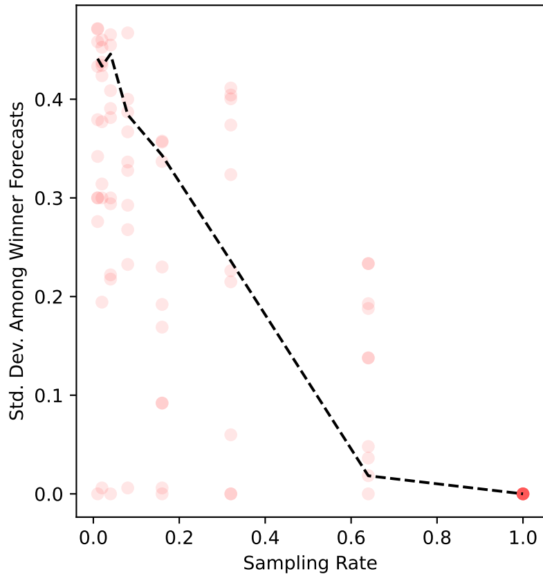
apa-10 Uncertainty
