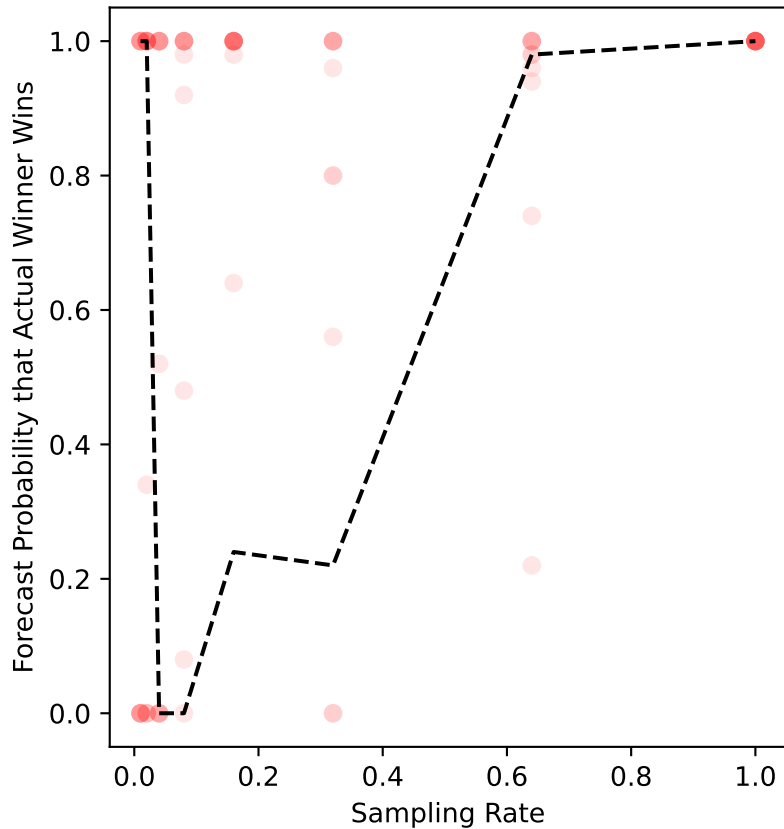
apa-10 Forecast
