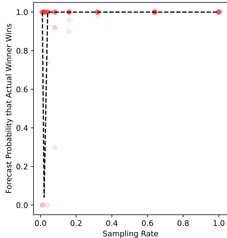
apa-11 Forecast
