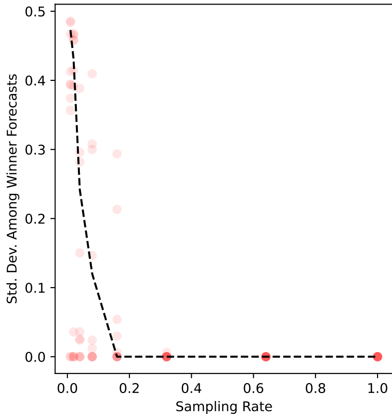
apa-11 Uncertainty
