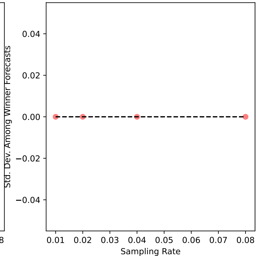
burlington-02 Uncertainty
