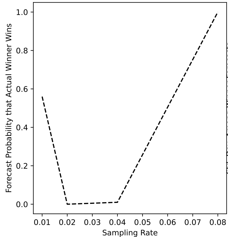
burlington-02 Forecast
