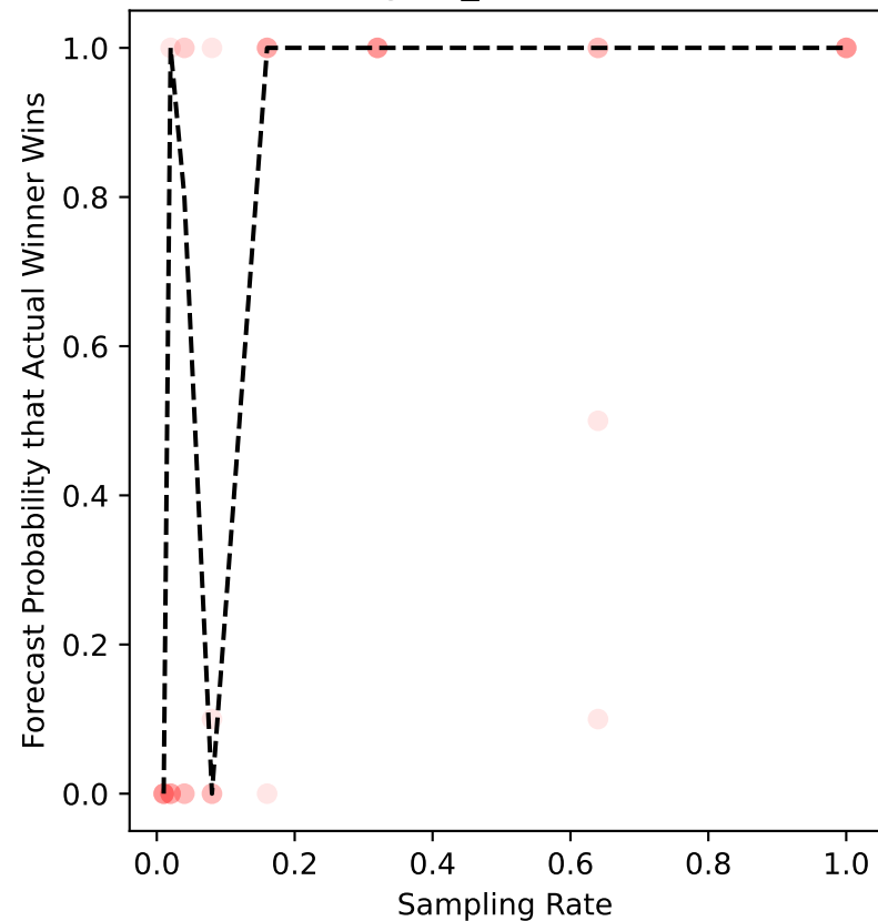
burlington_2009 Forecast
