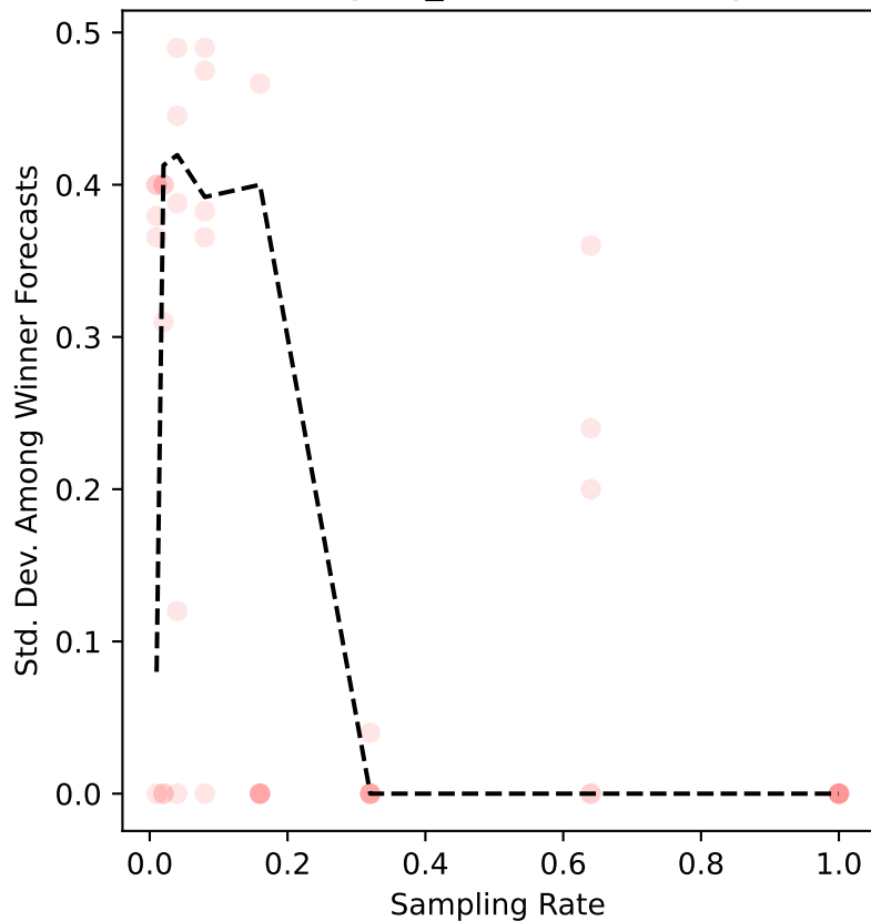
burlington_2009 Uncertainty
