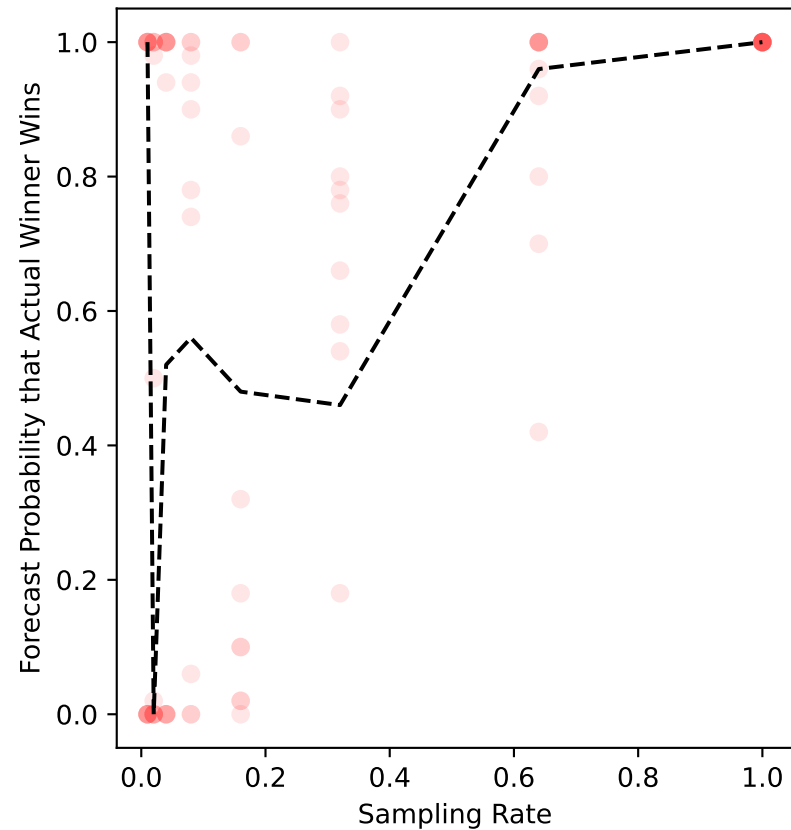
debian-02 Forecast
