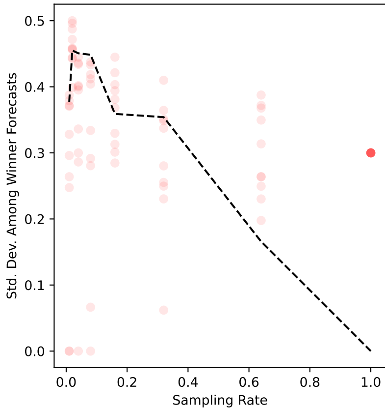
debian-02 Uncertainty
