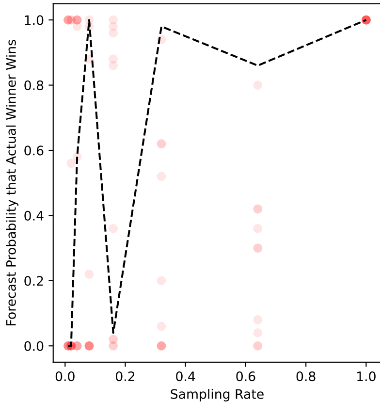
debian-03 Forecast
