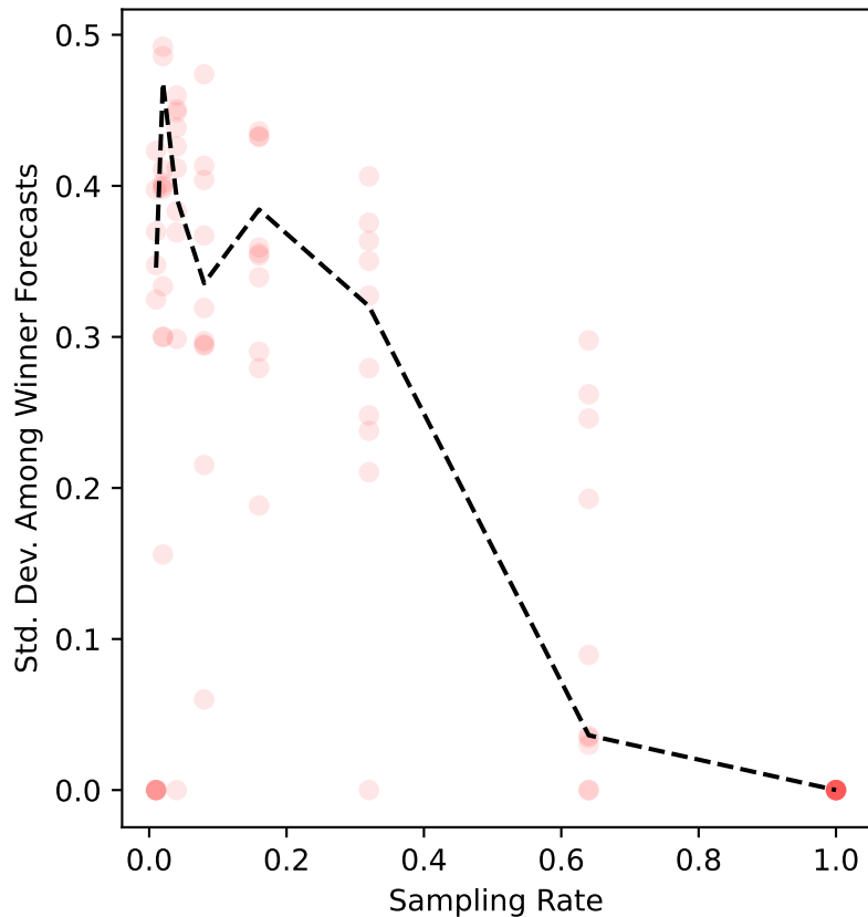
debian-05 Uncertainty
