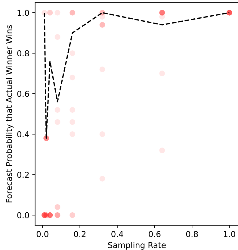
debian-08 Forecast
