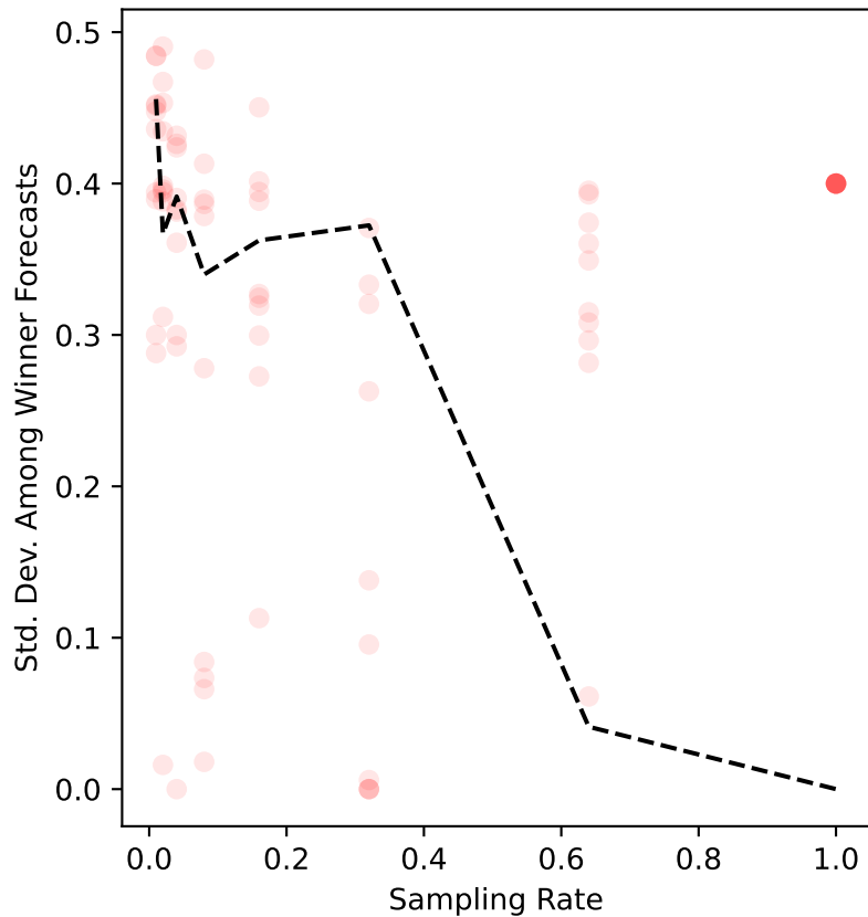
ers-13 Uncertainty
