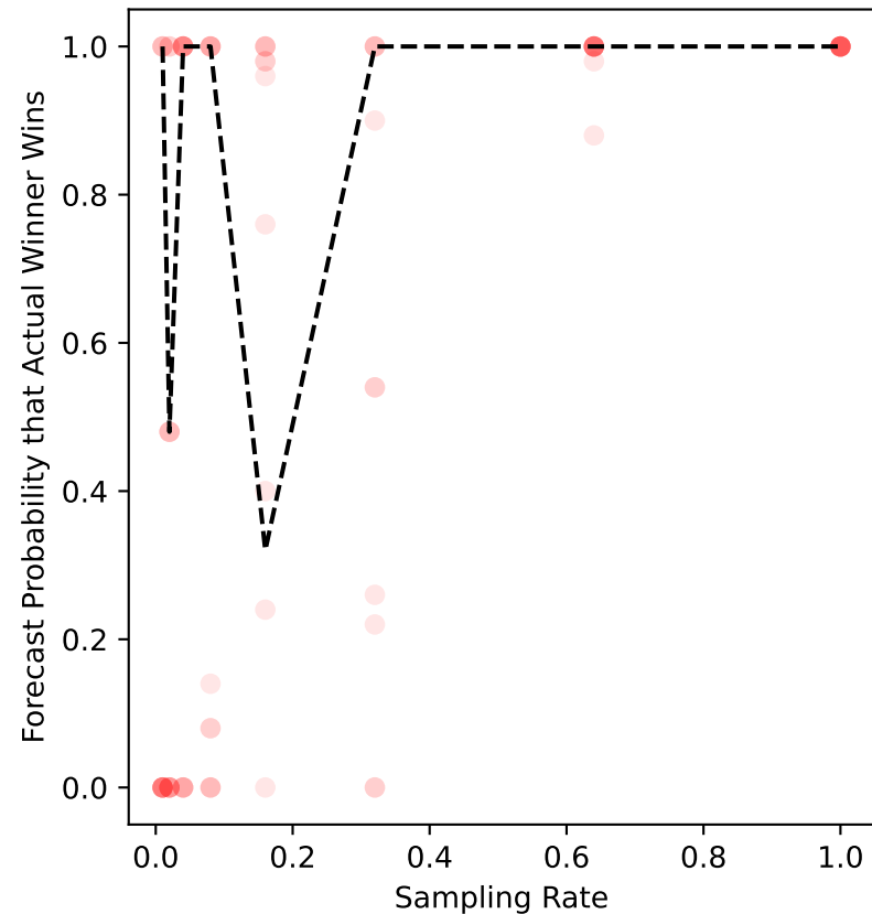
ers-74 Forecast
