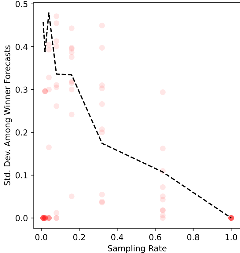
ers-74 Uncertainty
