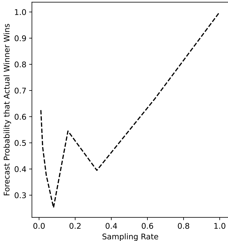
glasgow-04 Forecast
