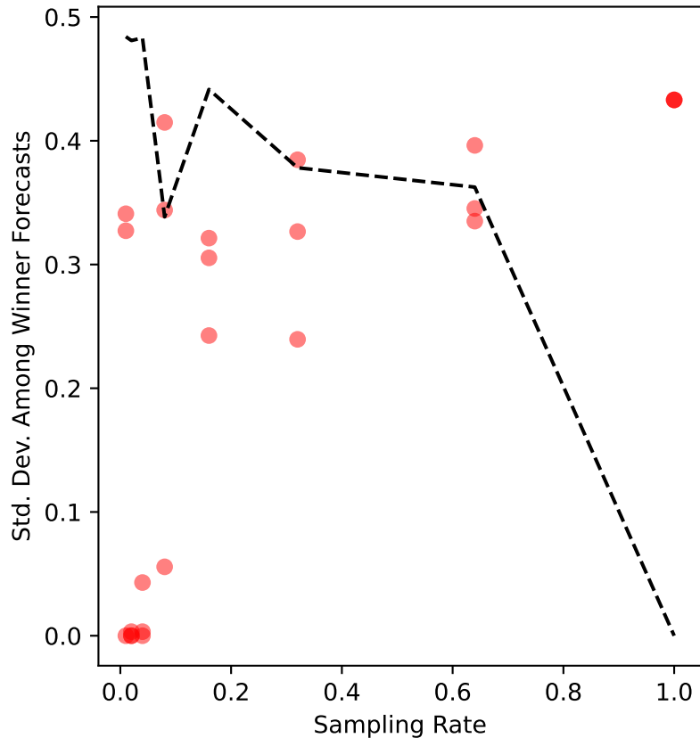
glasgow-04 Uncertainty
