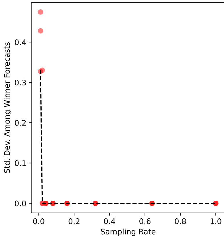
glasgow-08 Uncertainty
