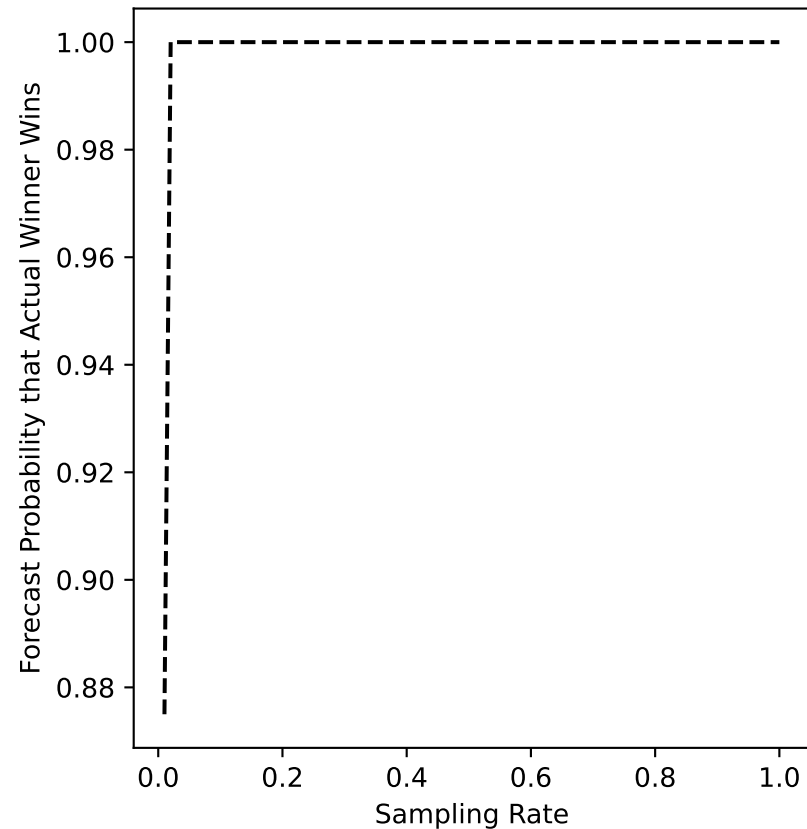
glasgow-08 Forecast
