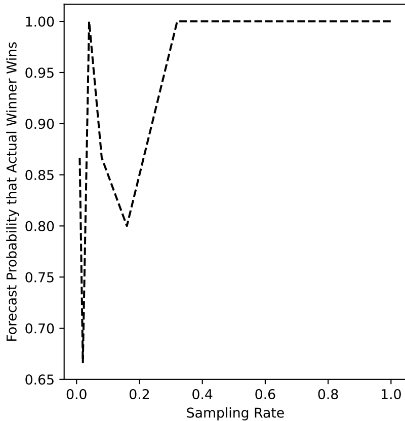
glasgow-11 Forecast
