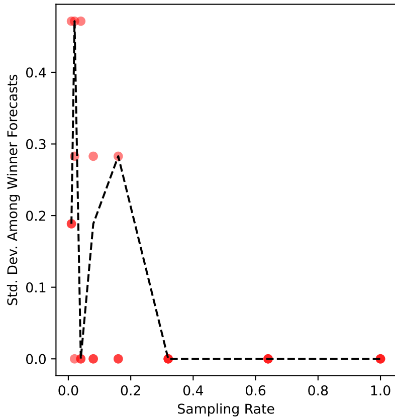
glasgow-11 Uncertainty
