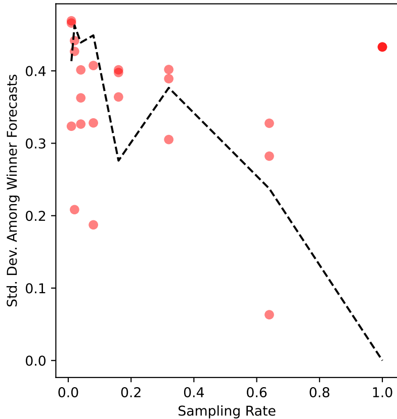
glasgow-12 Uncertainty
