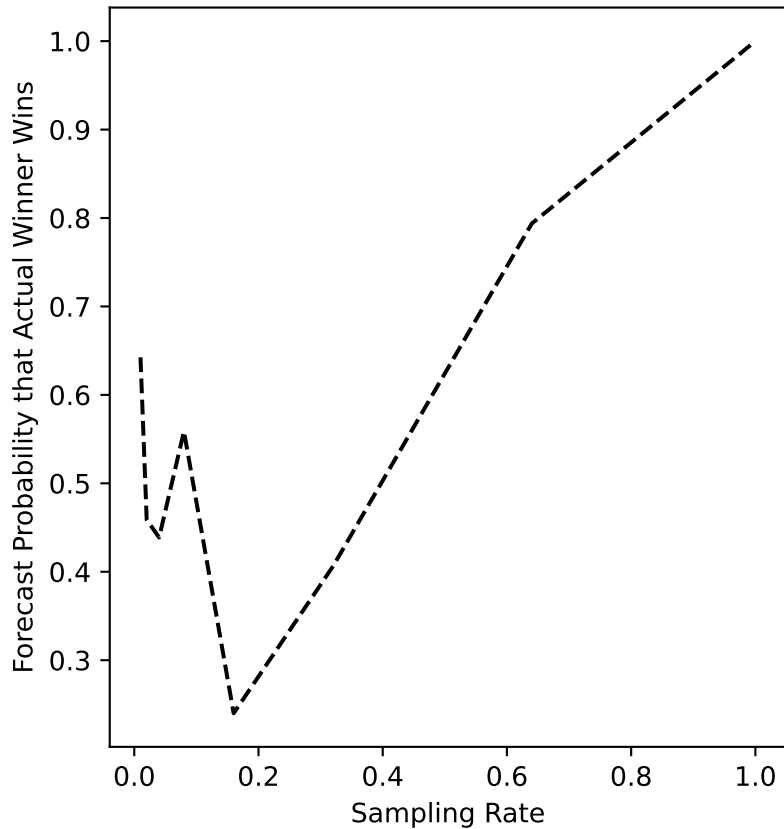
glasgow-12 Forecast
