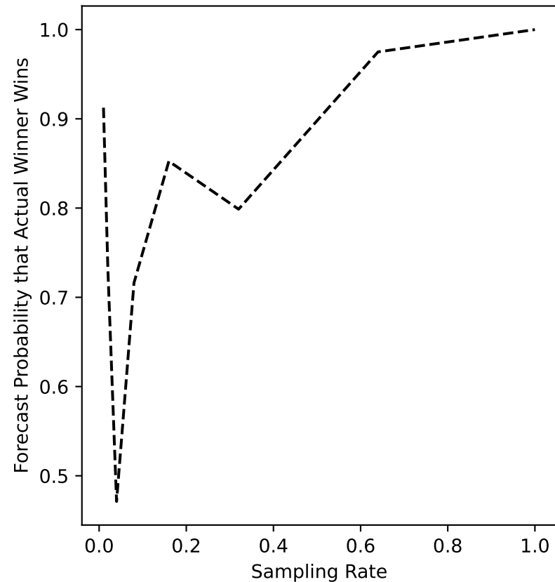
glasgow-14 Forecast
