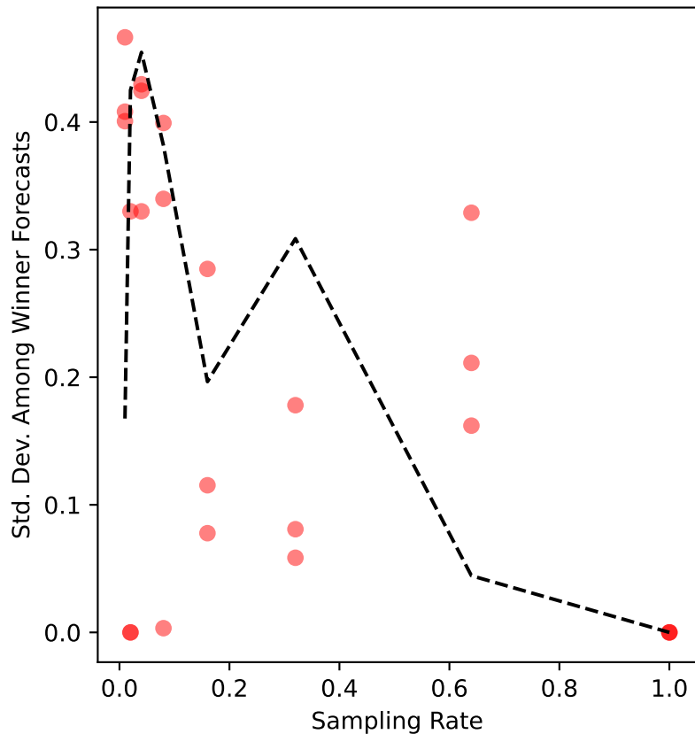
glasgow-14 Uncertainty
