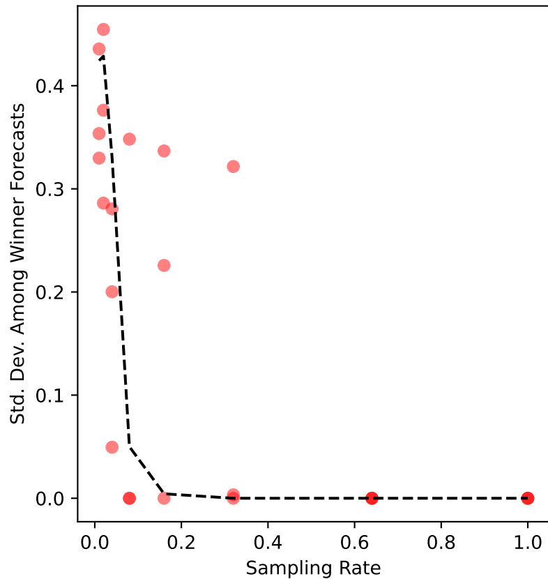
glasgow-18 Uncertainty
