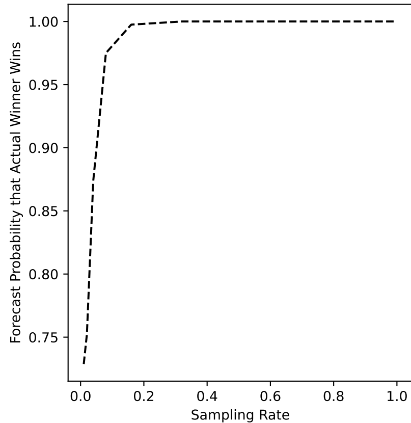
glasgow-18 Forecast
