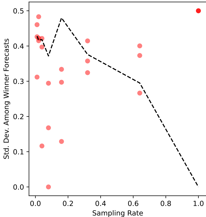
glasgow-20 Uncertainty
