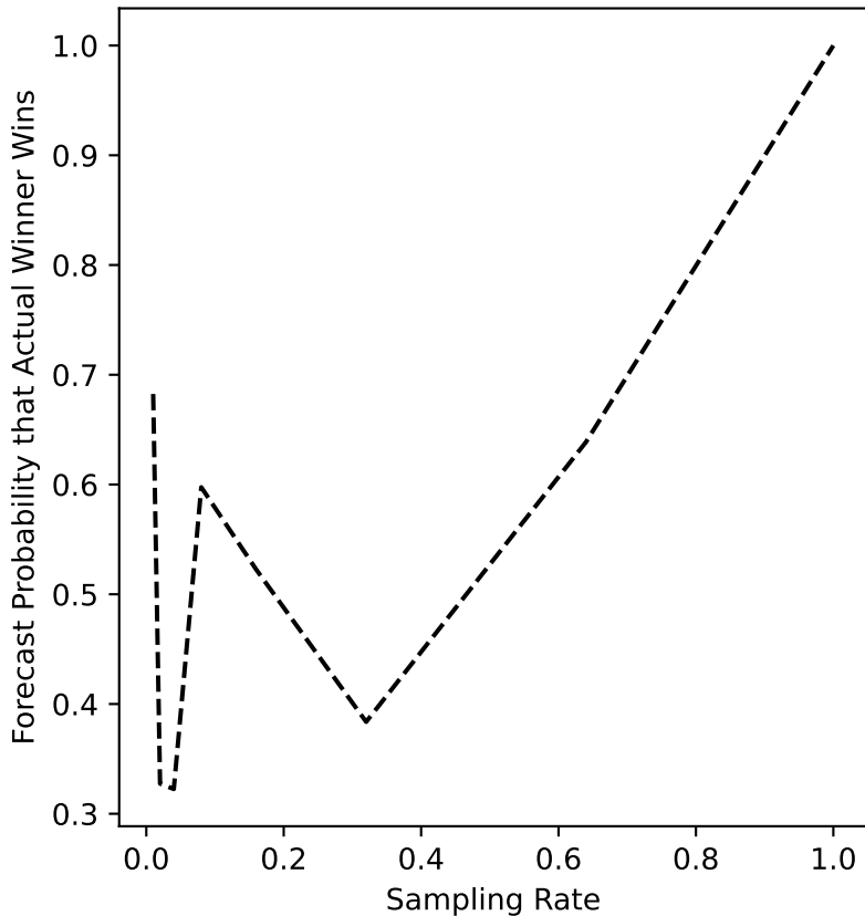
glasgow-20 Forecast
