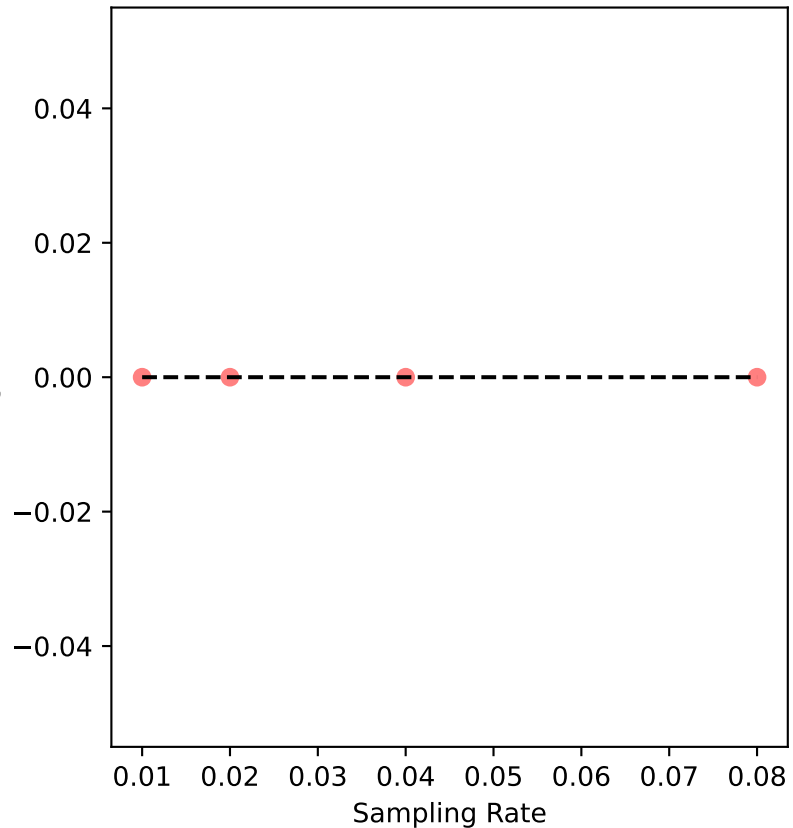
minneapolis-04 Uncertainty
