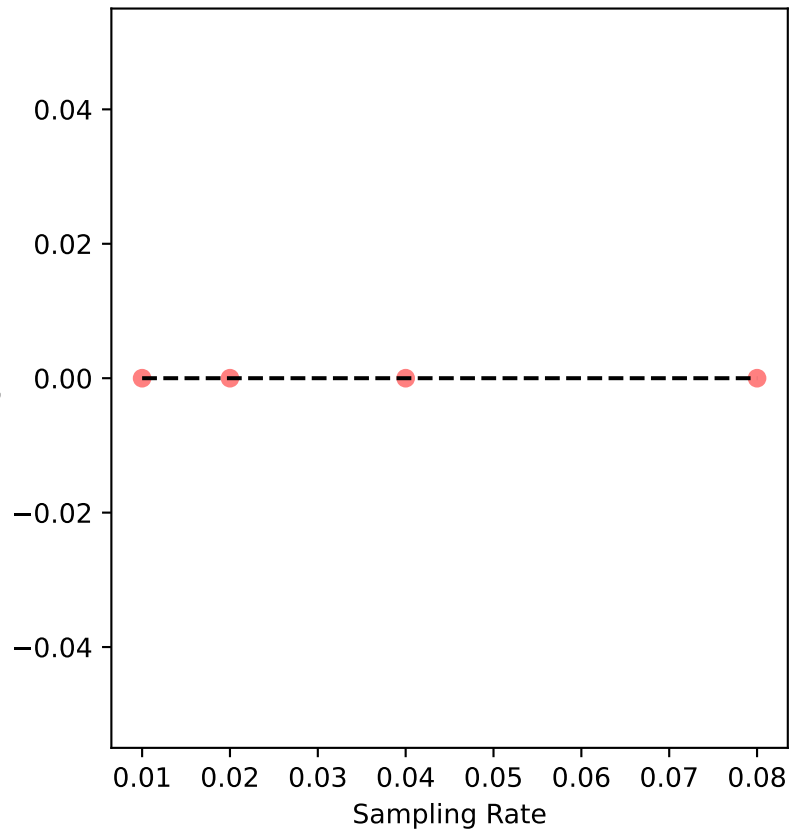
oakland-04 Uncertainty
