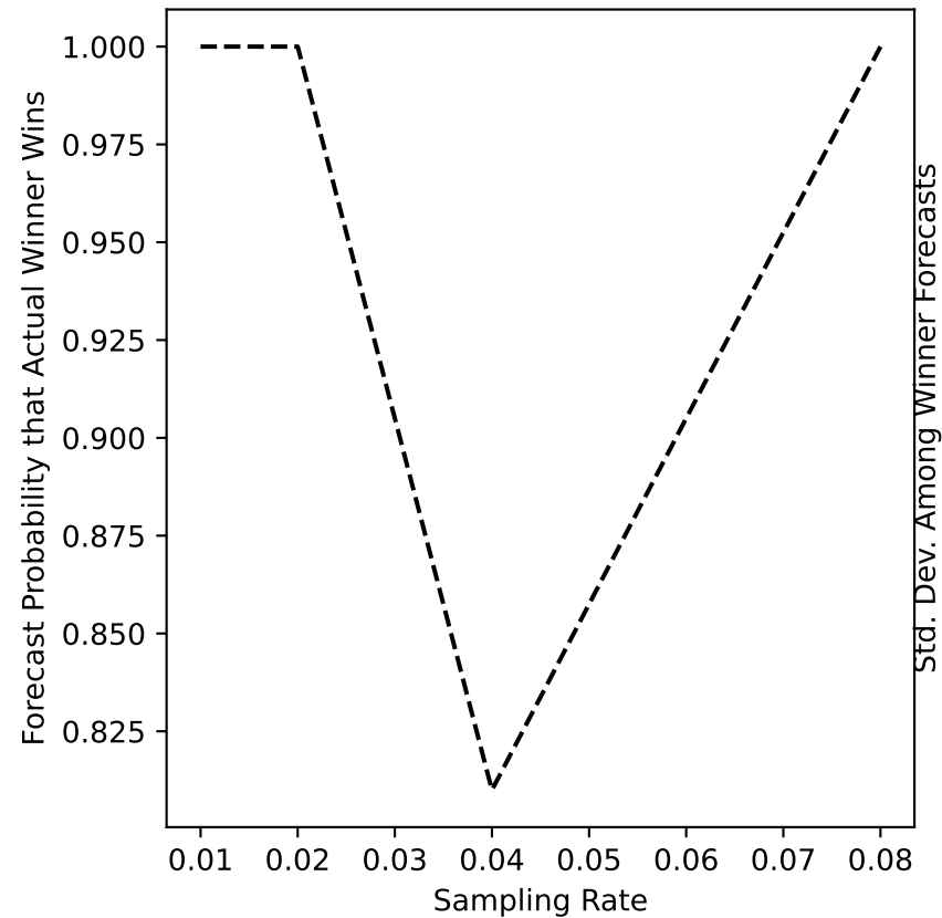
oakland-04 Forecast
