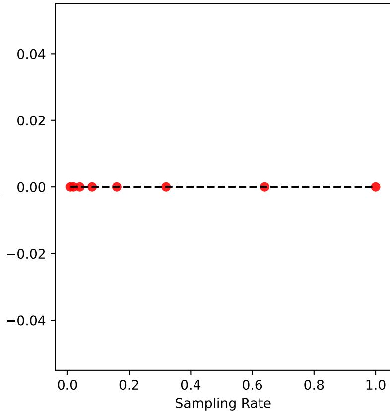
sf-11 Uncertainty
