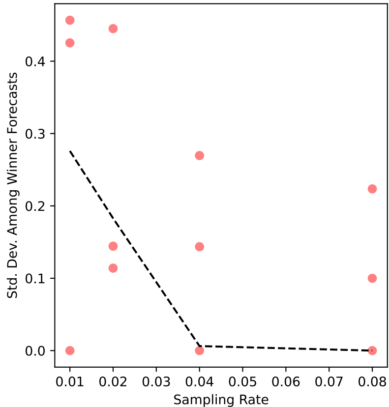
berkley-01 Uncertainty
