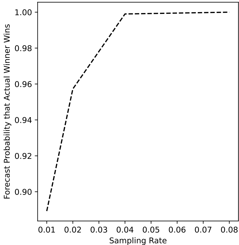
berkley-01 Forecast
