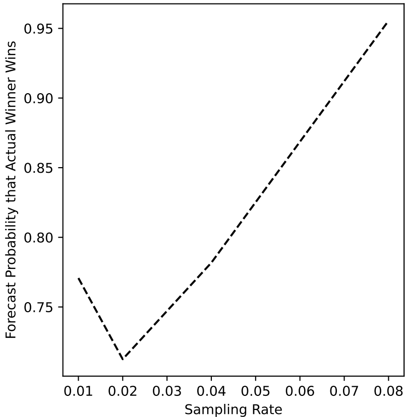
minneapolis-02 Forecast
