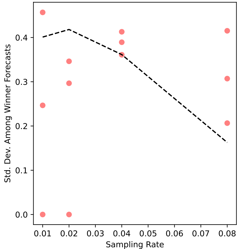
minneapolis-02 Uncertainty
