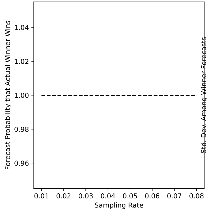
oakland-01 Forecast
