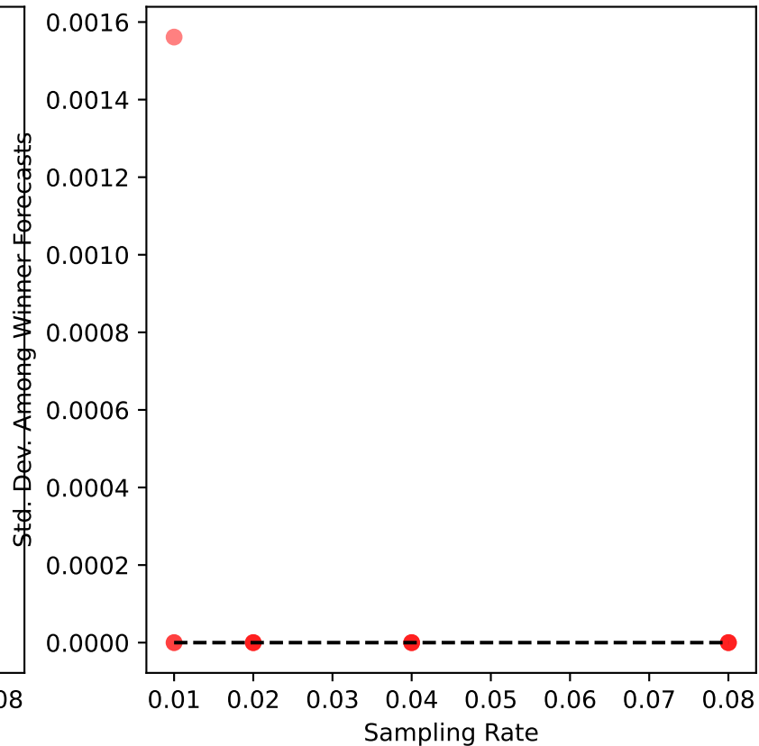
oakland-01 Uncertainty
