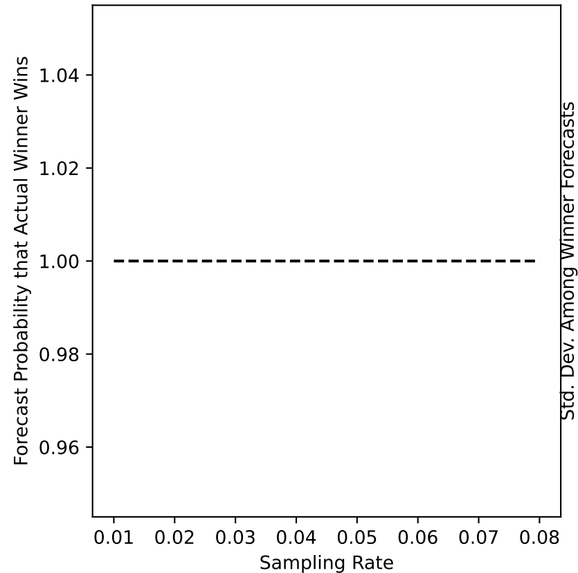
oakland-03 Forecast
