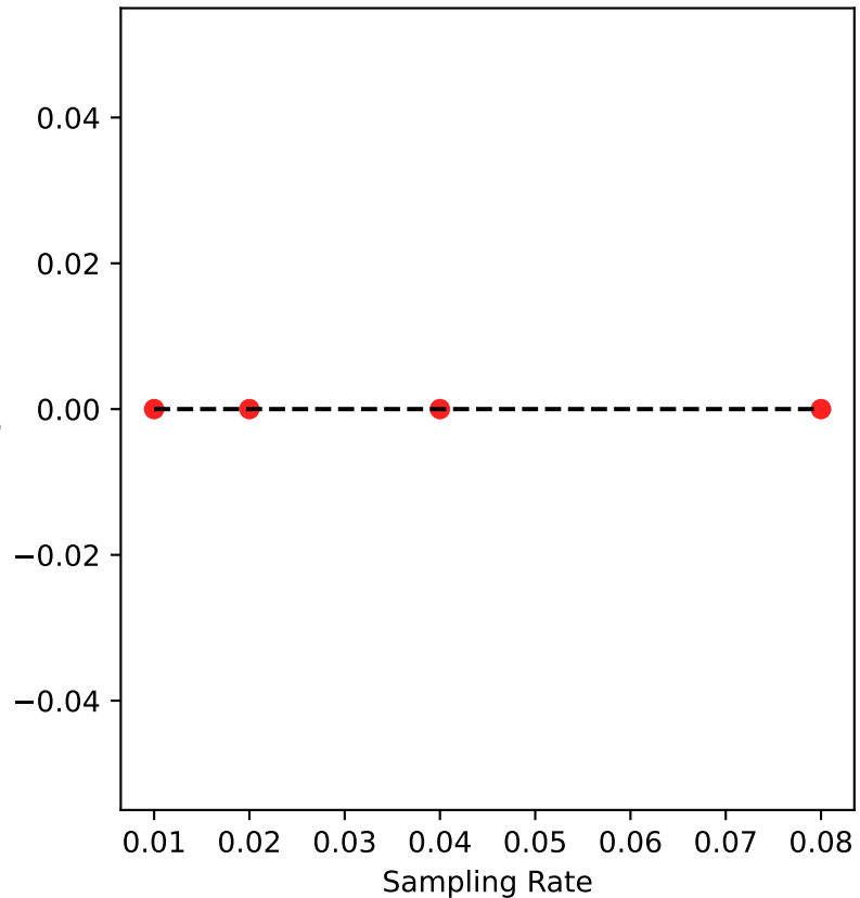
oakland-03 Uncertainty
