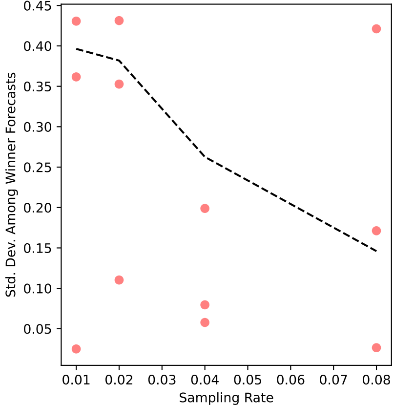
oakland-05 Uncertainty
