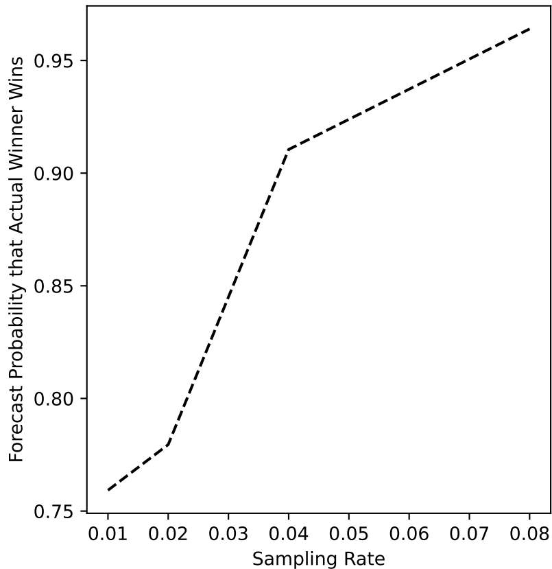
oakland-05 Forecast
