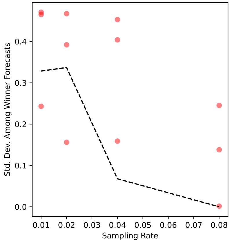
pierce-03 Uncertainty
