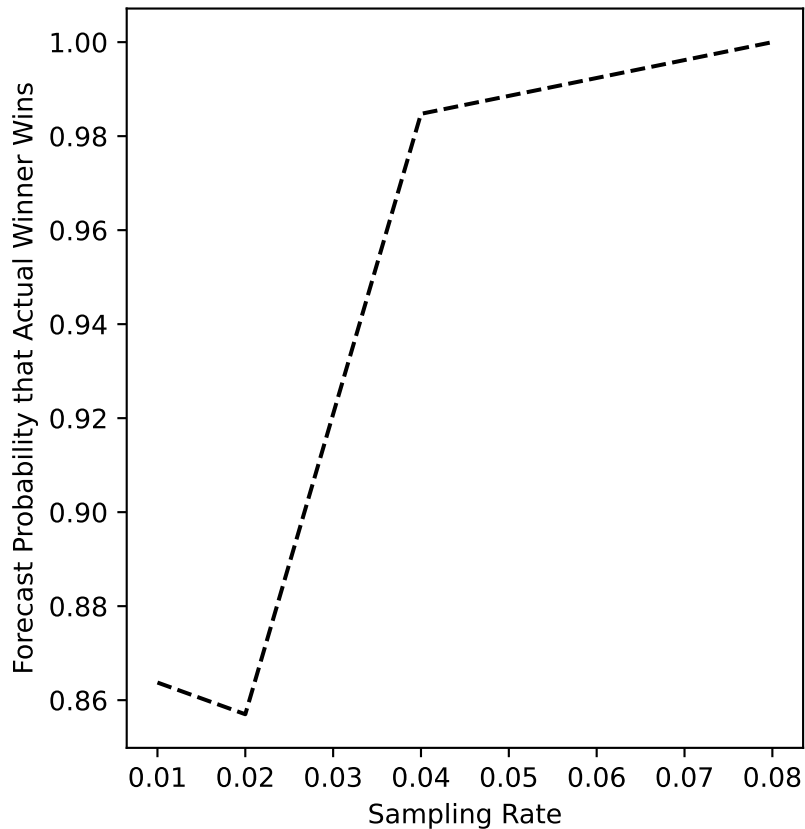
pierce-03 Forecast
