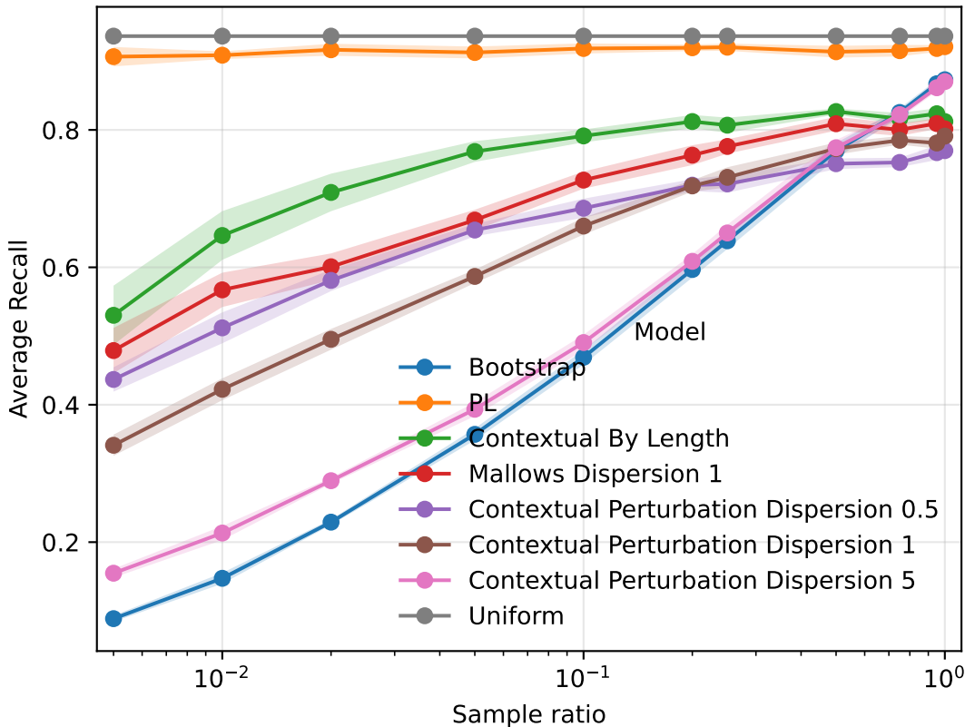
Recall vs. Sample Ratio by Model
