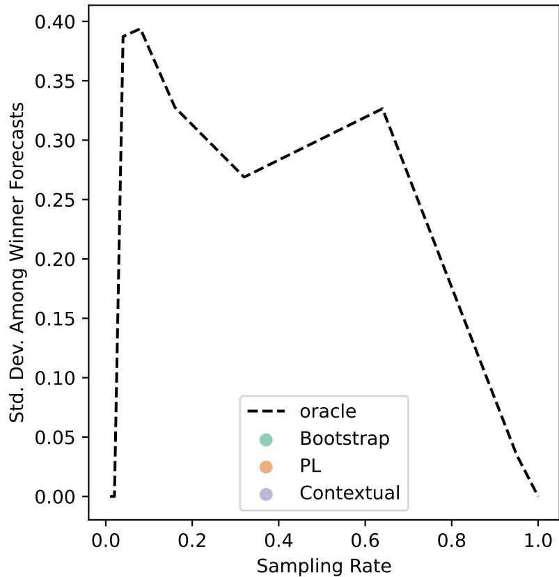
ers-07 Uncertainty
