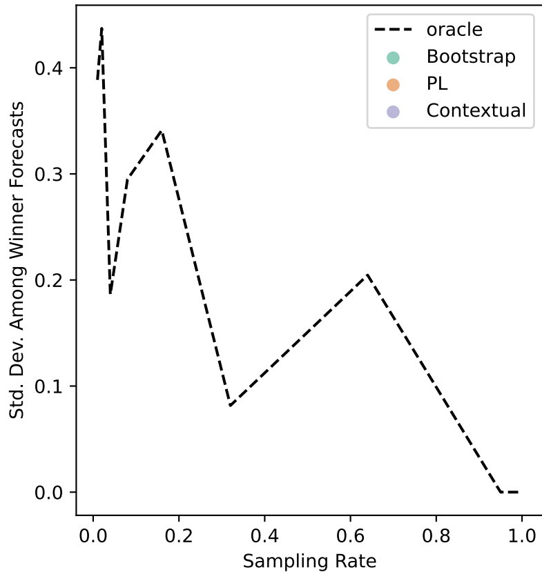
ers-12 Uncertainty
