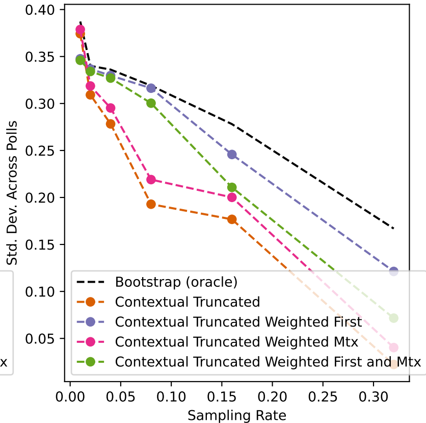
sf-01 Uncertainty
