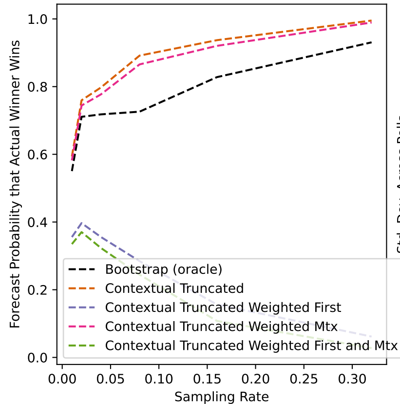
sf-01 Forecast
