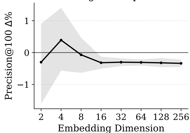
LastFM-Asia Target Group: 0
