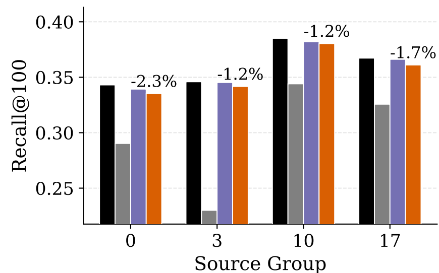
LastFM-Asia Matrix Factorization
