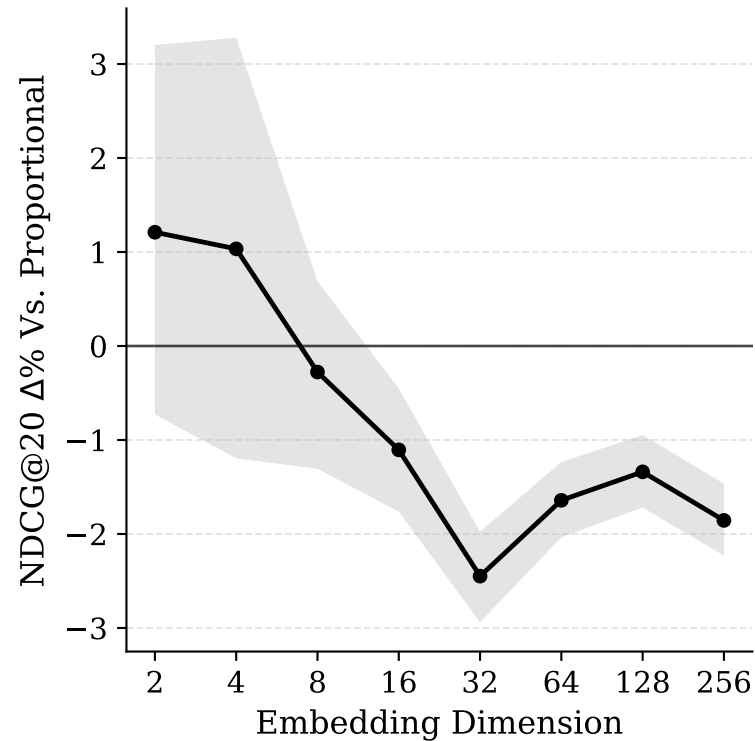
MovieLens-1M Source Group: 45
