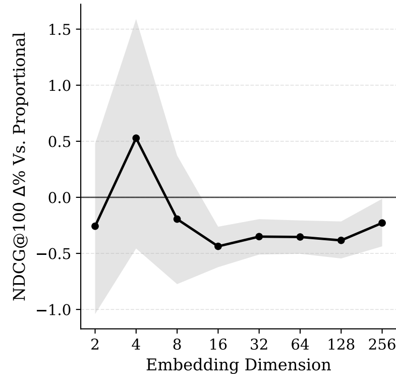
LastFM-Asia Source Group: 0
