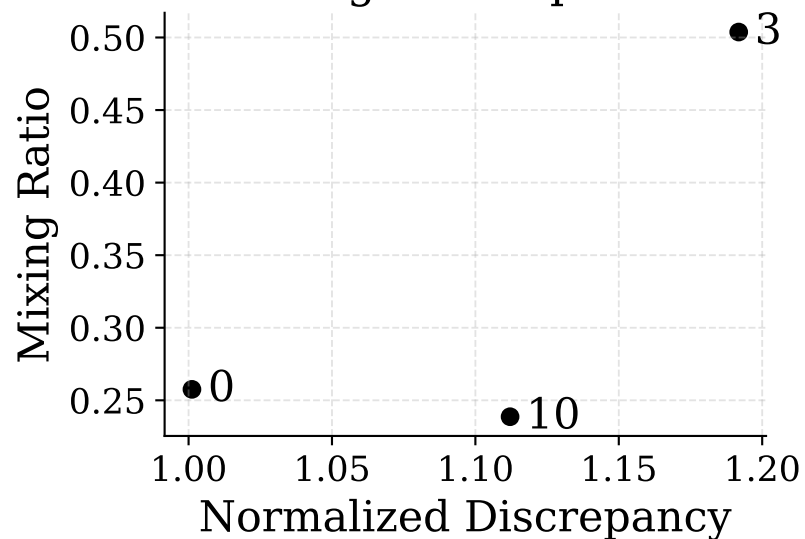
LastFM-Asia Target Group: 17
