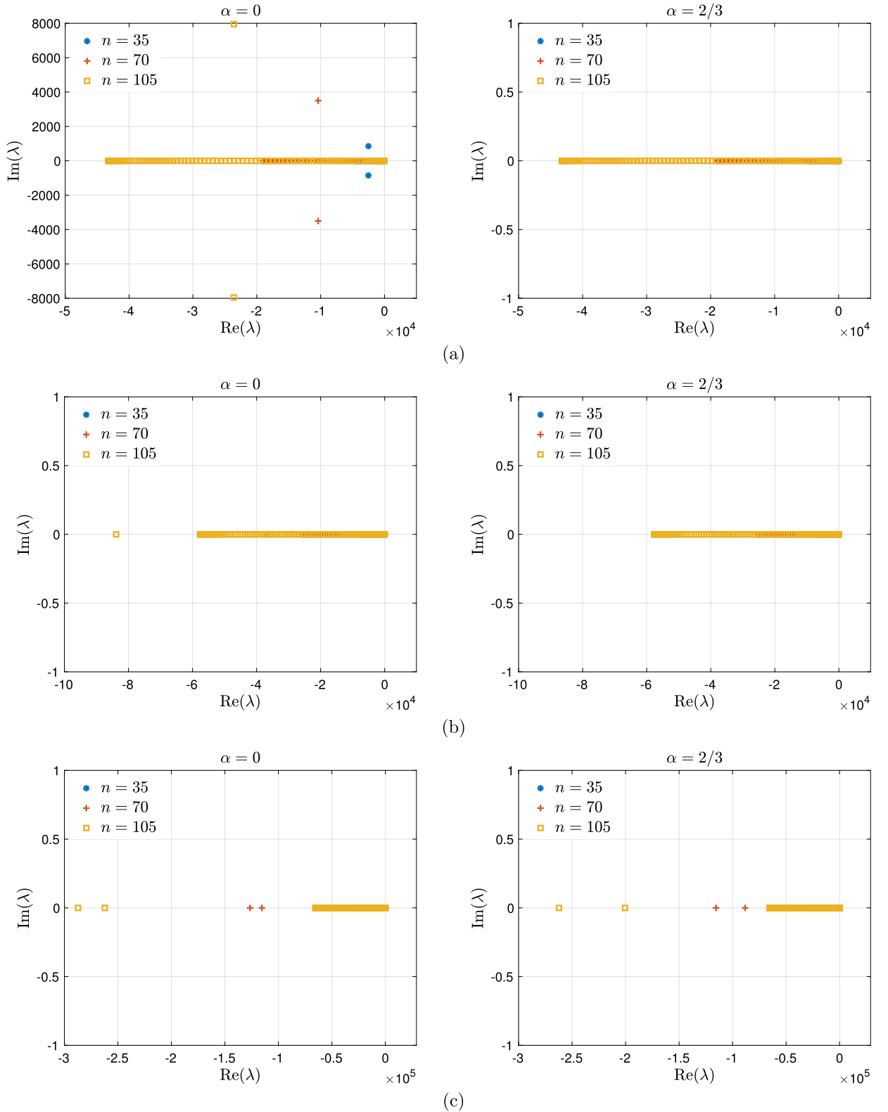
Fig. 6. Eigenvalue spectra of the system matrix to solve the one-dimensional diffusion problem of section 5.2 using (a) D_2^{p=1} , (b) D_2^{p=2} , and (c) D_2^{p=3} for \alpha = 0 (left column) and \alpha = 2/3 (right column) over a domain as shown in Fig. 2 with various number of grid points. Note the difference in axis limits for various D_2^p operators.
