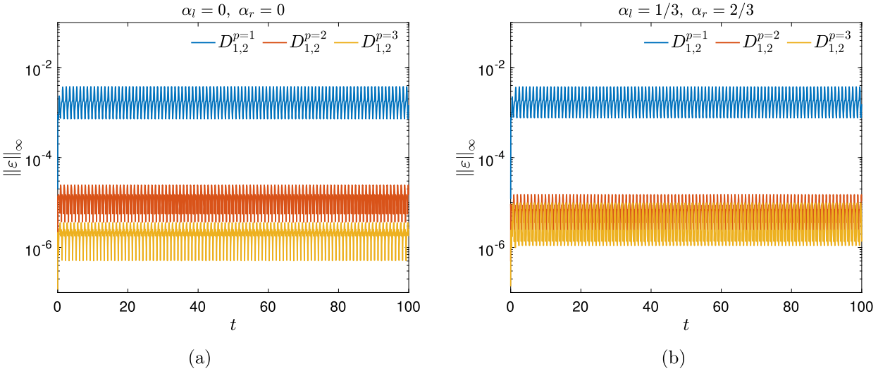
Fig. 11. L_\infty -error from the long-time simulations of (52) with the initial condition (55) and the boundary condition (58). Semi-discretization (59) is used over the grid shown in Fig. 8 with 80 grid points and (a) \alpha_l = \alpha_r = 0 , and (b) \alpha_l = 1/3 , \alpha_r = 2/3 .
