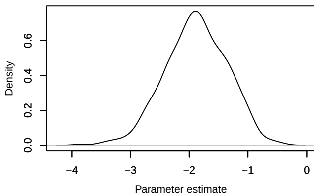
Density – alpha0[3]
