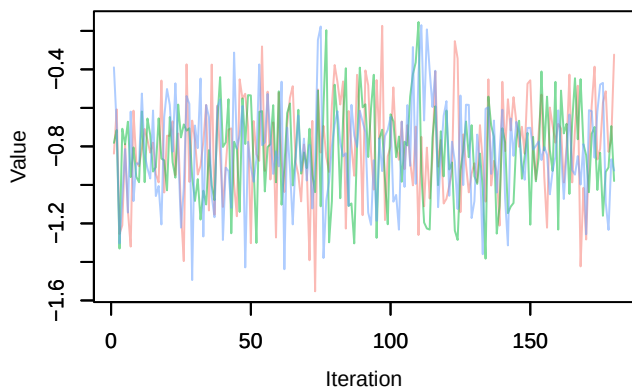
Trace – alpha0[7]
