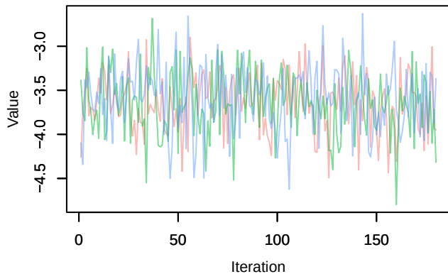
Trace – alpha0[15]
