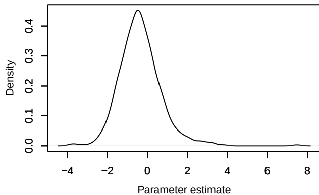
Density – beta.ranef.categ.in_AP[15,2]
