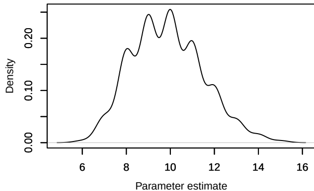
Density – Nspecies_station[25]
