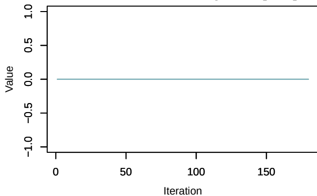
Trace – beta.ranef.categ.in_AP[20,1]
