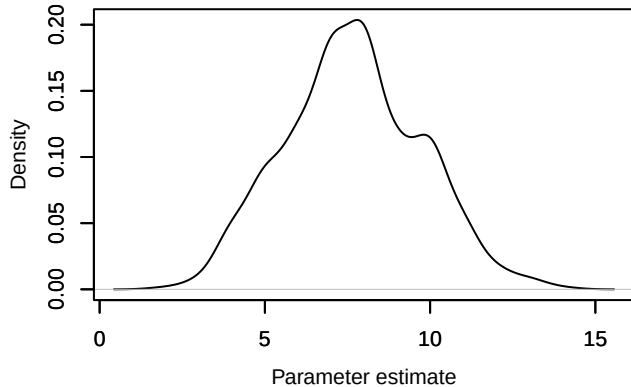
Density – Nspecies_station[41]
