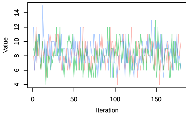
Trace – Nspecies_station[2]
