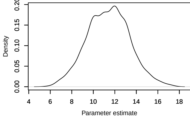
Density – Nspecies_station[11]
