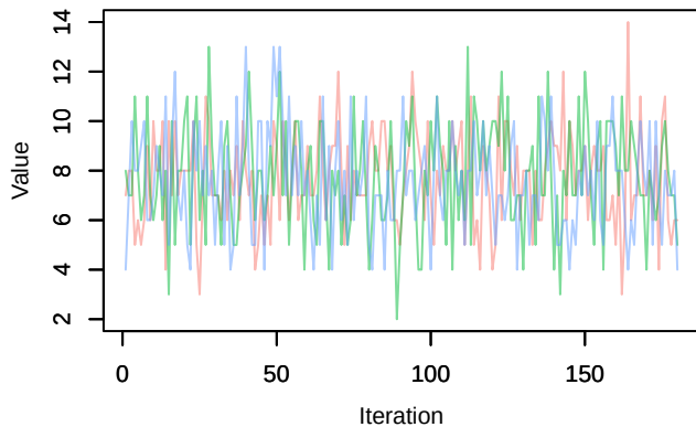
Trace – Nspecies_station[41]
