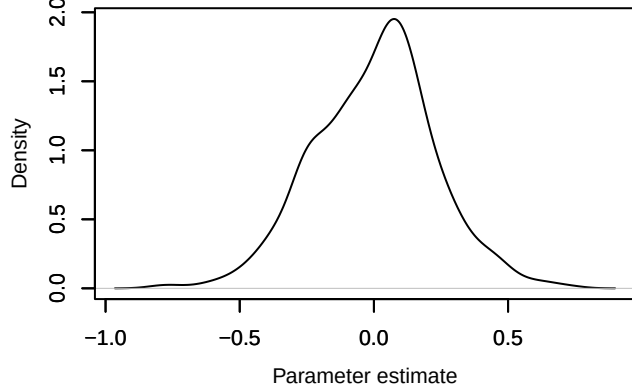
Density – beta.ranef.cont.elev[5]
