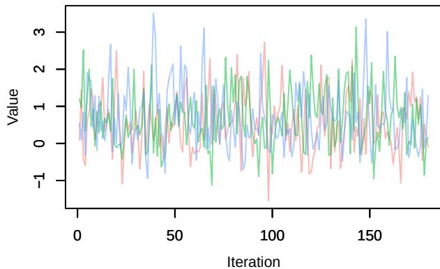
Trace – beta.ranef.cont.border_dist[18]
