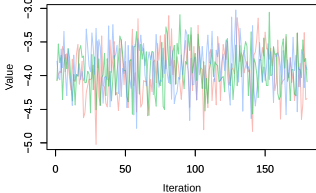
Trace – alpha0[13]
