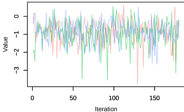
Trace – beta.ranef.cont.border_dist[19]
