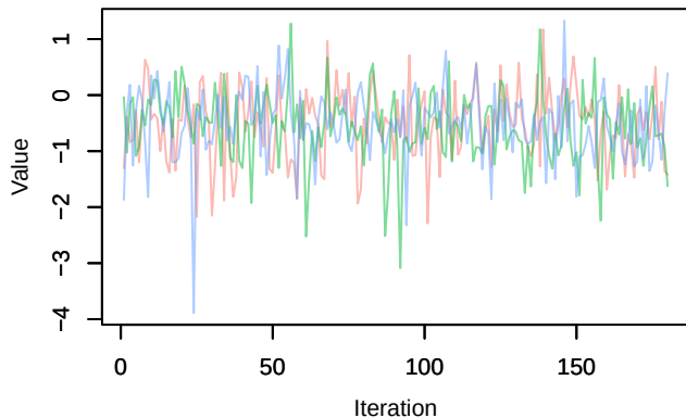
Trace – beta.ranef.cont.border_dist[13]
