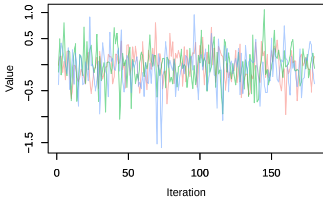
Trace – beta.ranef.cont.elev[15]
