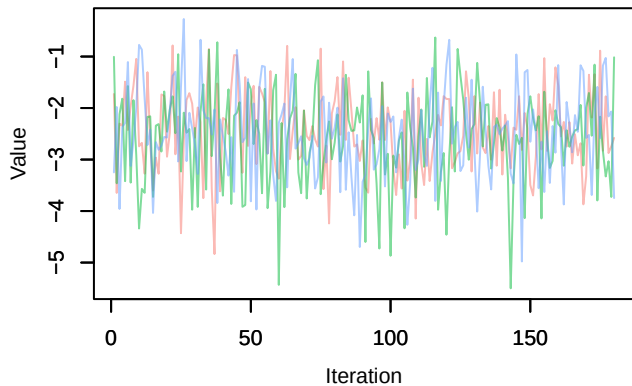
Trace – alpha0[12]
