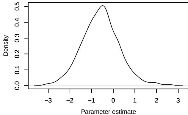
Density – beta.ranef.categ.in_AP[19,2]
