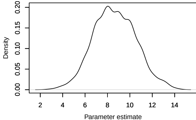
Density – Nspecies_station[58]
