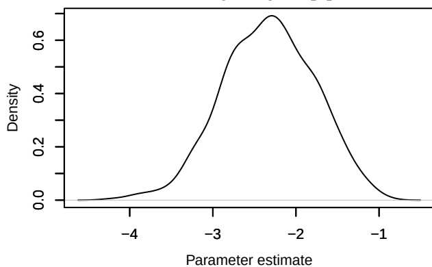
Density – alpha0[6]
