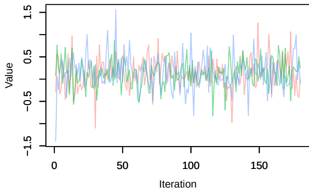
Trace – beta.ranef.cont.elev[12]
