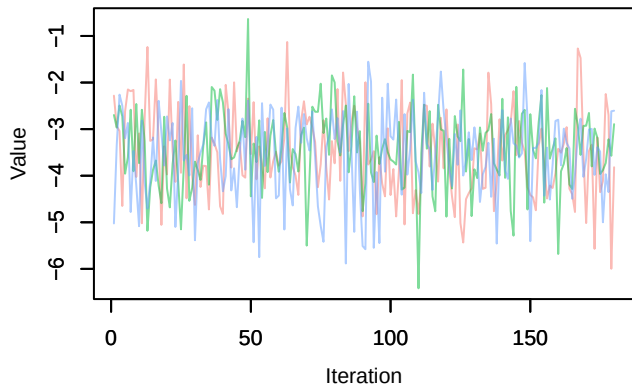
Trace – alpha0[13]
