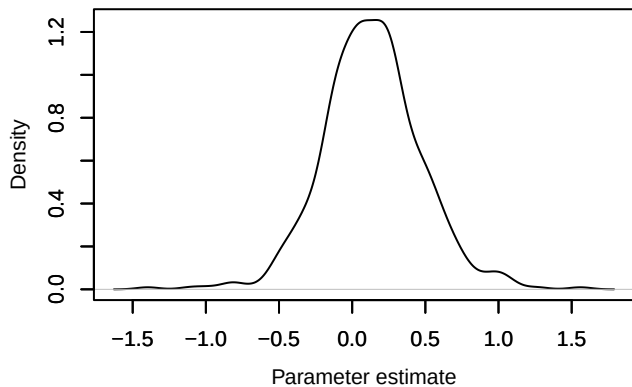
Density – beta.ranef.cont.elev[12]
