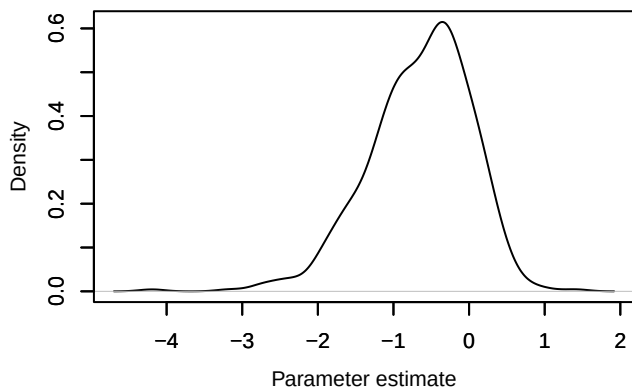
Density – beta.ranef.cont.border_dist[7]
