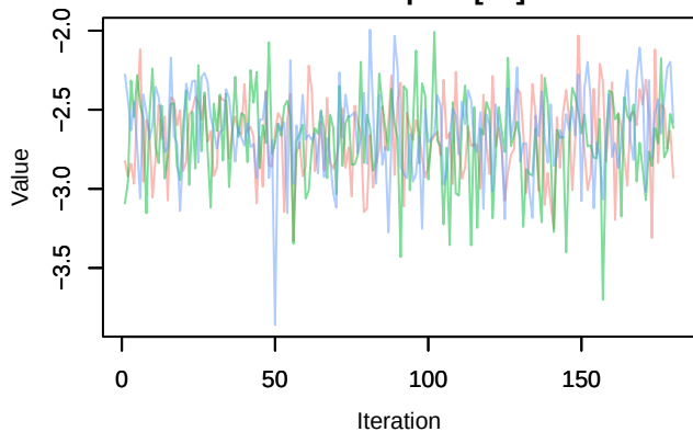
Trace – alpha0.mean
