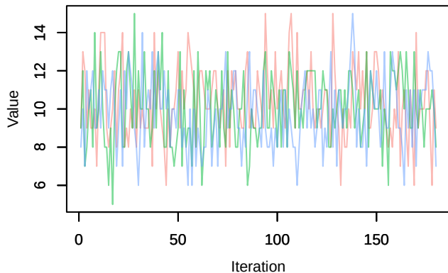
Trace – Nspecies_station[44]
