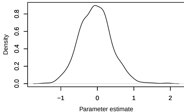
Density – beta.ranef.cont.border_dist[3]
