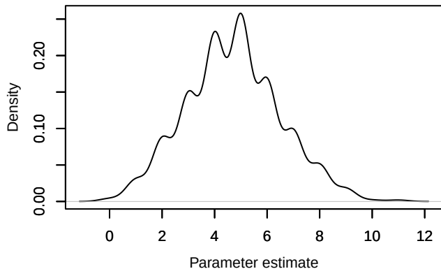
Density – Nspecies_station[4]
