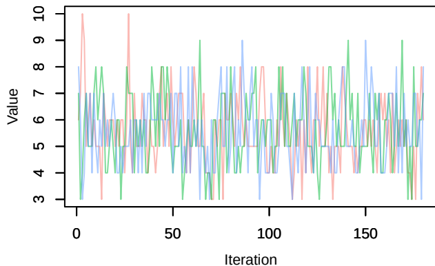
Trace – Nspecies_station[38]
