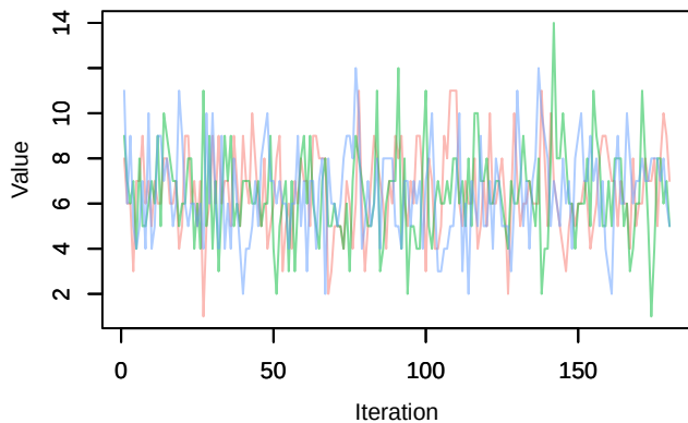
Trace – Nspecies_station[62]
