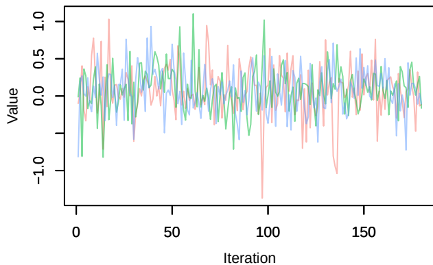
Trace – beta.ranef.cont.elev[18]
