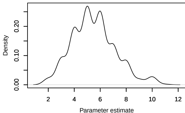
Density – Nspecies_station[34]
