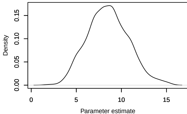
Density – alpha.obs.fixed.cont.effort
