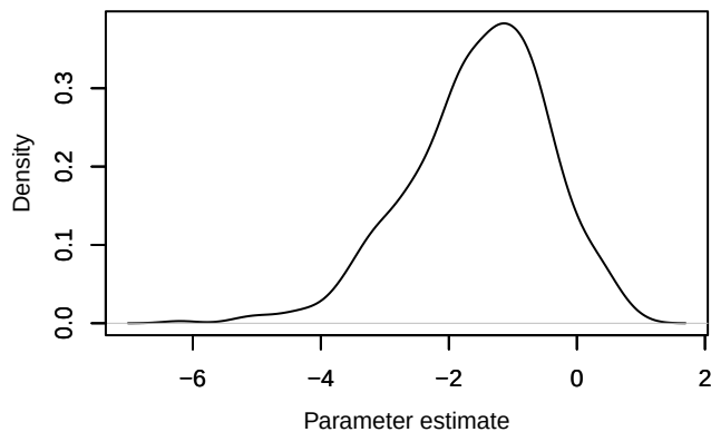
Density – beta.ranef.categ.in_AP[12,2]
