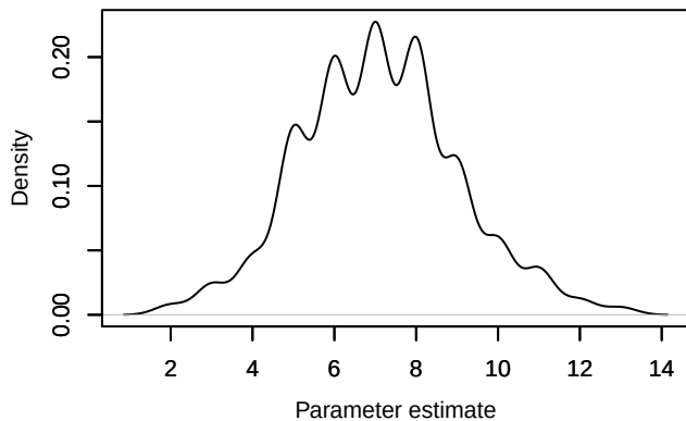
Density – Nspecies_station[32]
