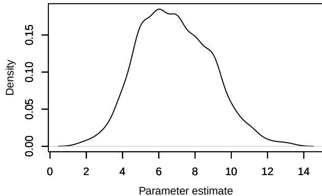
Density – Nspecies_station[44]
