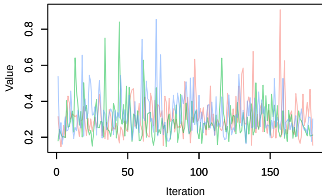
Trace – beta0[1]
