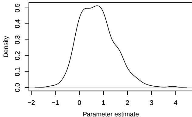
Density – beta.ranef.cont.border_dist[16]
