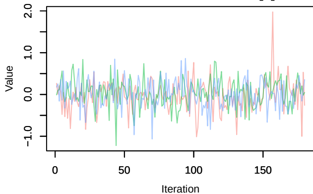
Trace – beta.ranef.cont.elev[8]
