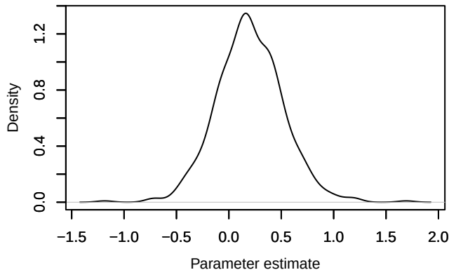
Density – beta.ranef.cont.elev[12]
