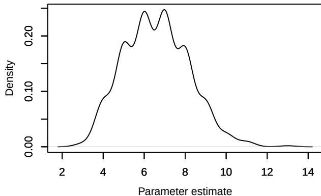
Density – Nspecies_station[38]
