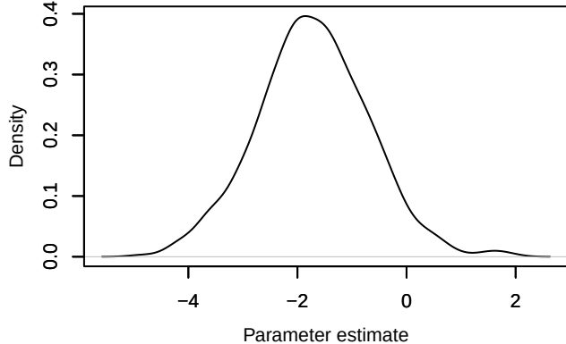
Density – beta0[11]
