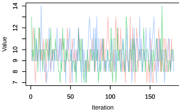
Trace – Nspecies_station[5]
