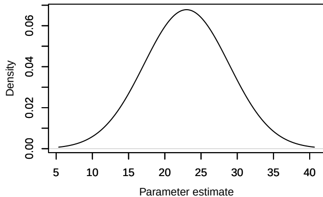
Density – Nspecies_station[1]
