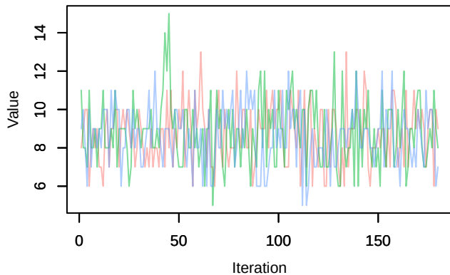
Trace – Nspecies_station[22]
