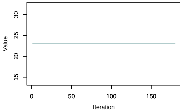
Trace – Nspecies_station[1]
