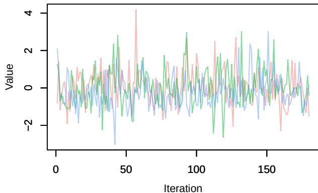
Trace – beta0[17]
