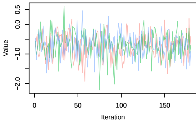
Trace – beta.ranef.cont.border_dist[4]
