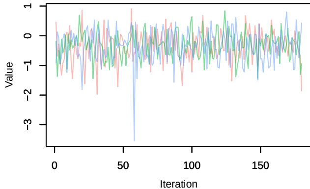
Trace – beta.ranef.cont.border_dist[22]
