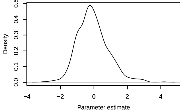
Density – beta0[17]
