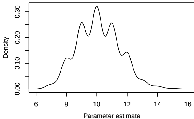
Density – Nspecies_station[35]
