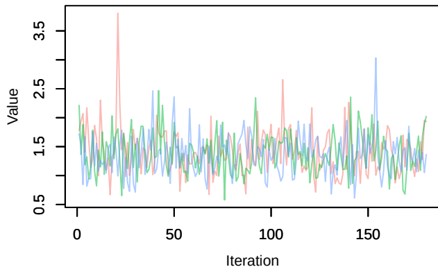
Trace – beta0.sigma
