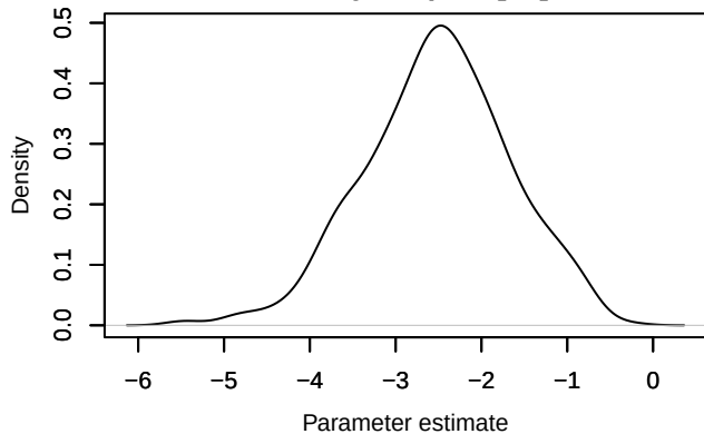
Density – alpha0[12]
