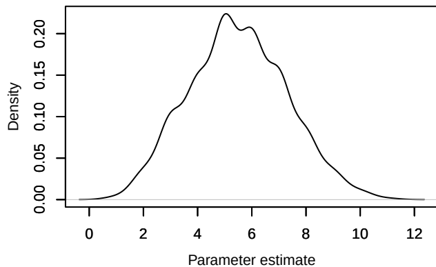
Density – Nspecies_station[50]
