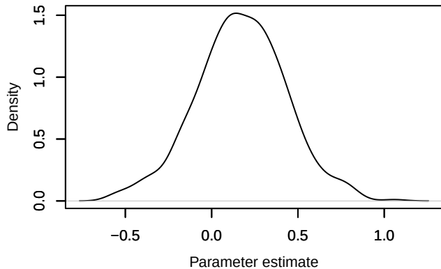
Density – beta.ranef.cont.elev[2]
