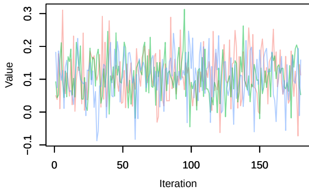
Trace – alpha0[1]
