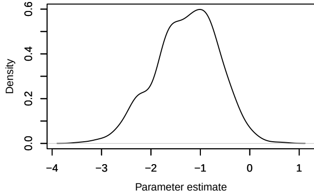
Density – beta0[7]
