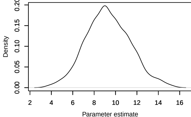
Density – Nspecies_station[41]
