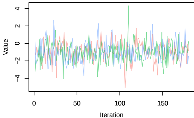
Trace – beta0[13]
