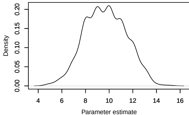
Density – Nspecies_station[49]
