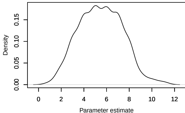
Density – Nspecies_station[7]
