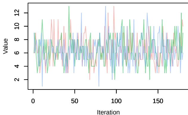
Trace – Nspecies_station[58]
