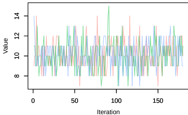
Trace – Nspecies_station[35]
