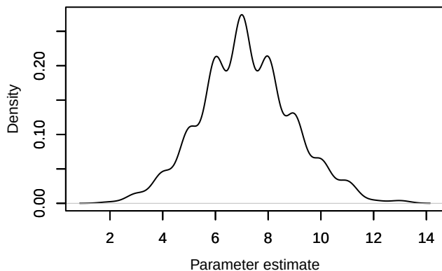
Density – Nspecies_station[52]
