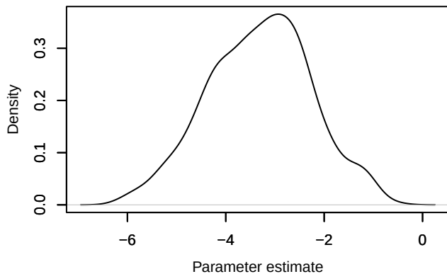
Density – alpha0[21]
