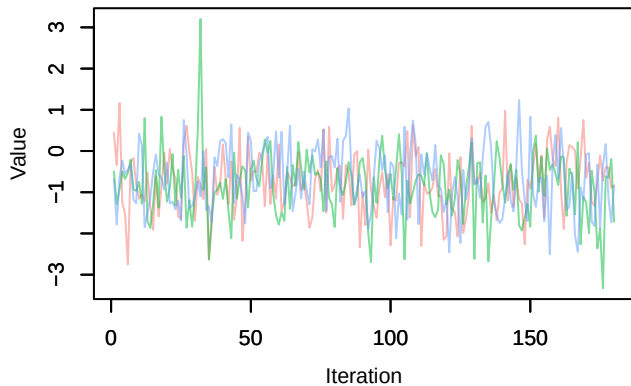
Trace – beta.ranef.categ.in_AP[3,2]
