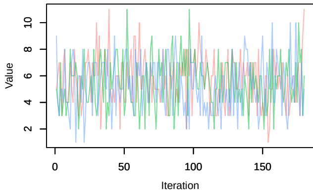
Trace – Nspecies_station[7]
