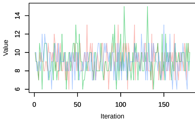
Trace – Nspecies_station[31]
