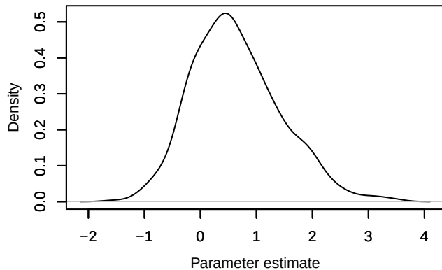
Density – beta.ranef.cont.border_dist[18]
