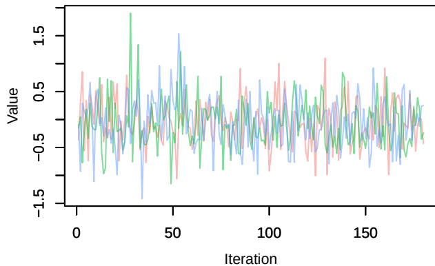
Trace – beta.ranef.cont.border_dist[3]
