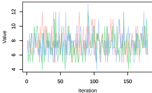
Trace – Nspecies_station[43]
