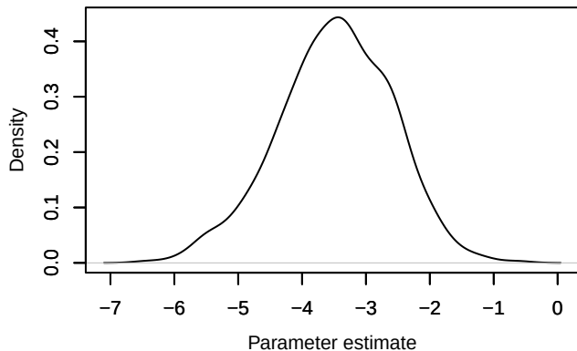
Density – alpha0[13]
