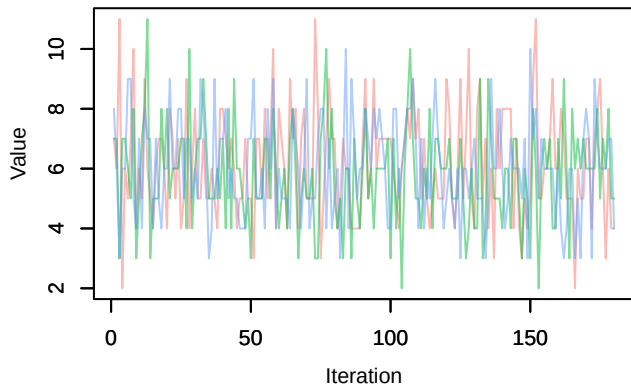
Trace – Nspecies_station[26]
