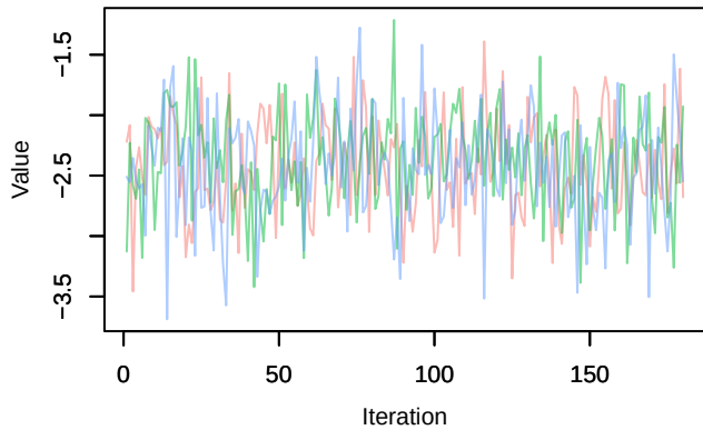
Trace – alpha0[22]
