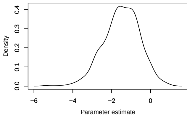
Density – beta.ranef.categ.in_AP[1,2]
