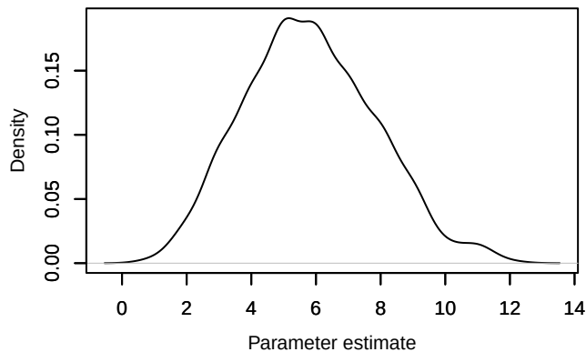
Density – Nspecies_station[20]
