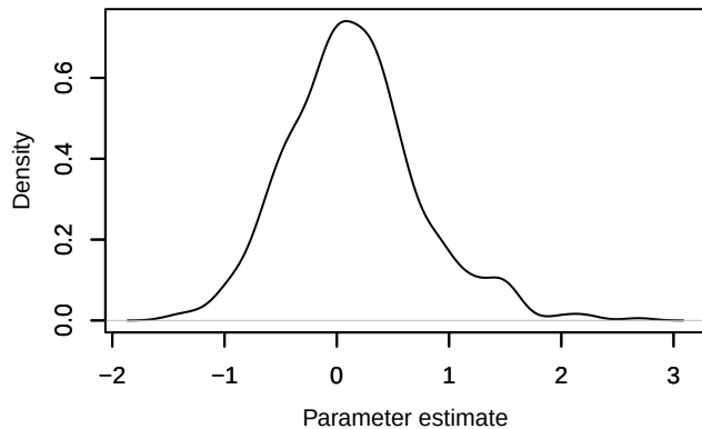
Density – beta.ranef.cont.border_dist[21]
