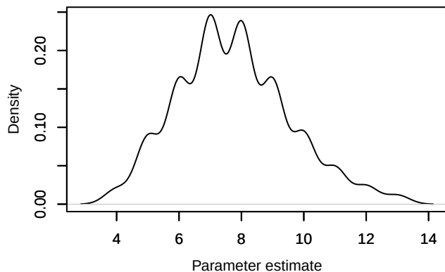
Density – Nspecies_station[61]
