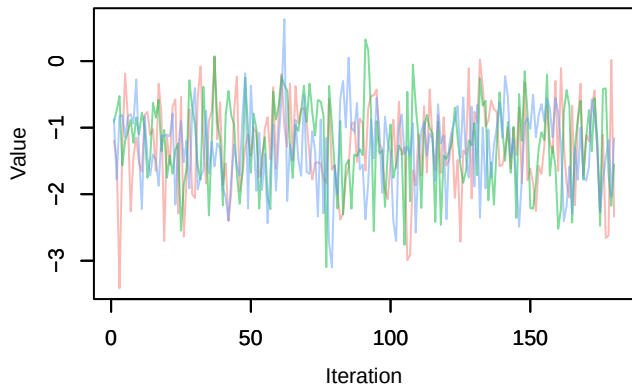
Trace – beta0[7]
