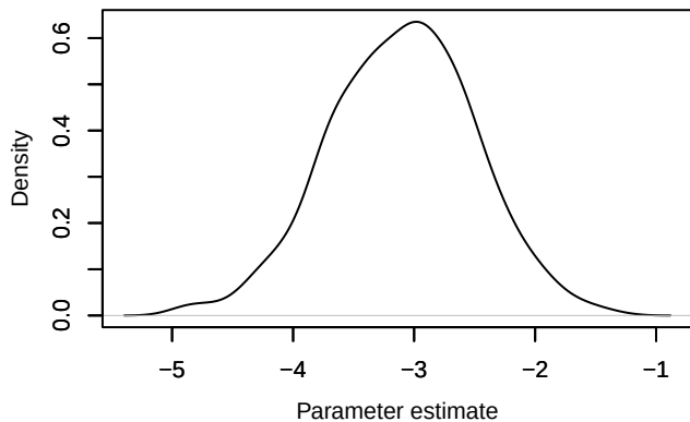
Density – alpha0[19]
