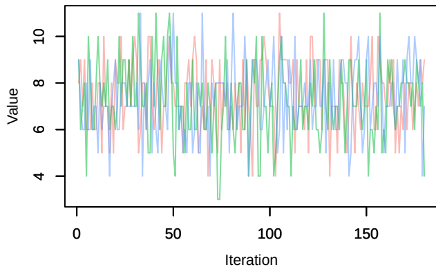
Trace – Nspecies_station[40]
