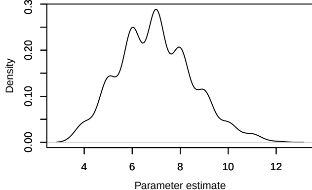
Density – Nspecies_station[29]
