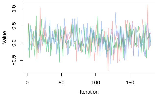
Trace – beta.ranef.cont.elev[3]
