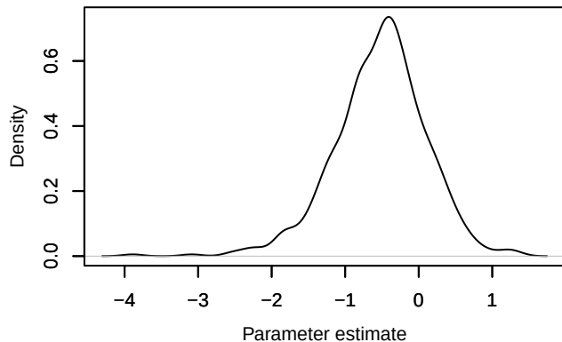
Density – beta.ranef.cont.border_dist[13]
