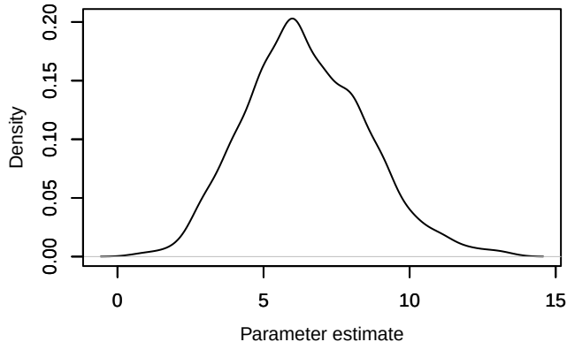
Density – Nspecies_station[58]
