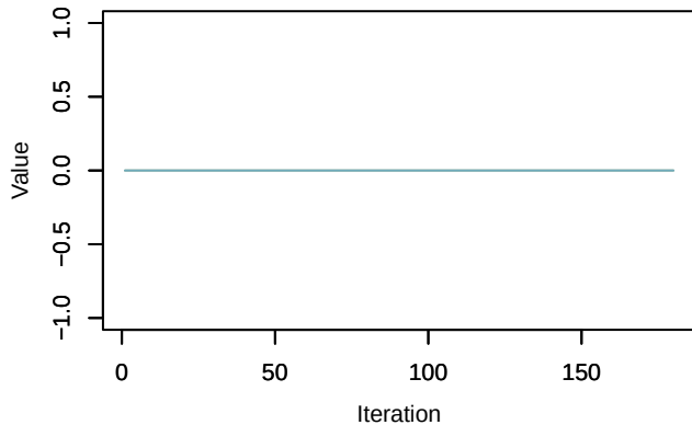
Trace – beta.ranef.categ.in_AP[2,1]
