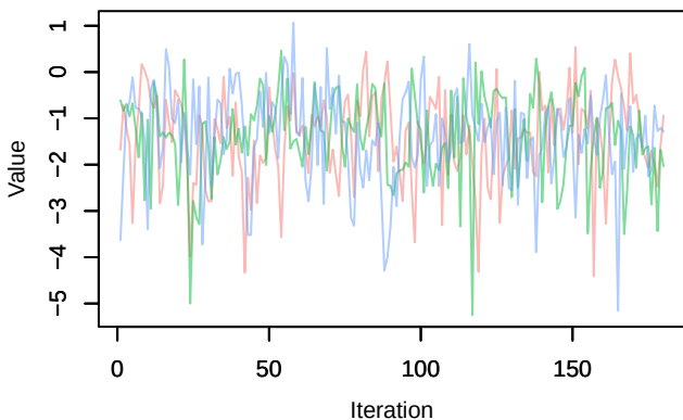
Trace – beta.ranef.category.in_AP[10,2]
