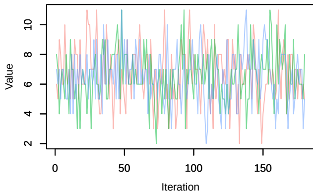
Trace – Nspecies_station[26]
