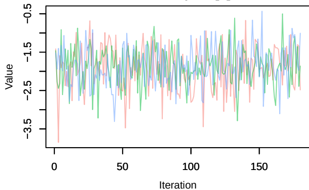
Trace – alpha0[3]
