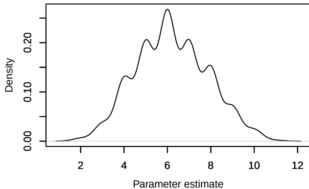
Density – Nspecies_station[46]
