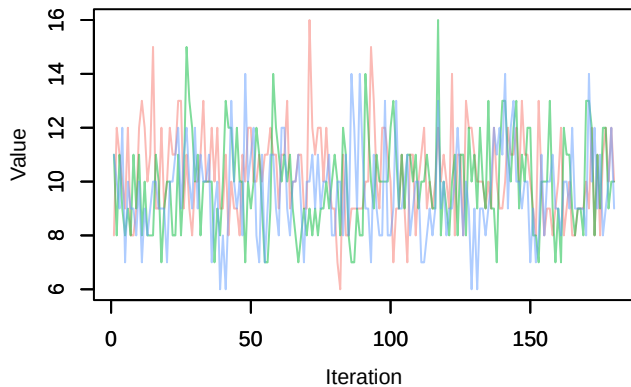
Trace – Nspecies_station[2]
