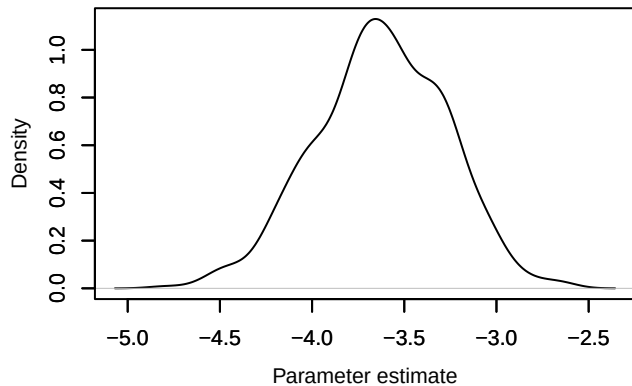
Density – alpha0[15]
