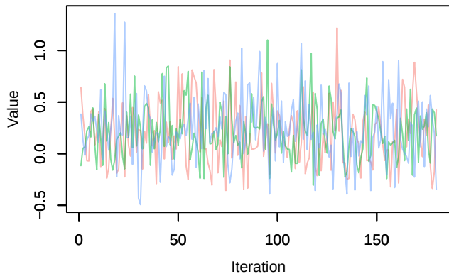
Trace – beta.ranef.cont.elev[11]
