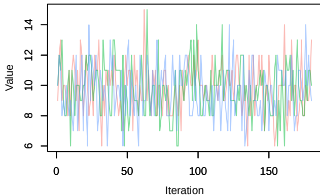
Trace – Nspecies_station[50]
