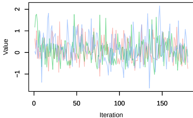
Trace – beta.ranef.cont.border_dist[12]
