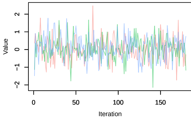
Trace – beta.ranef.cont.border_dist[15]
