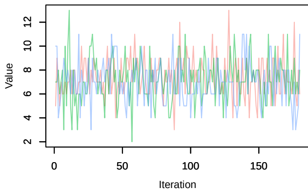
Trace – Nspecies_station[52]
