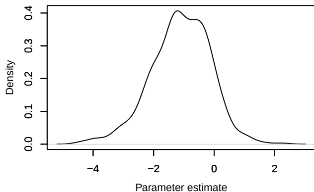
Density – beta.ranef.categ.in_AP[12,2]
