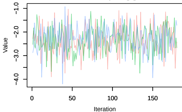
Trace – alpha0[6]
