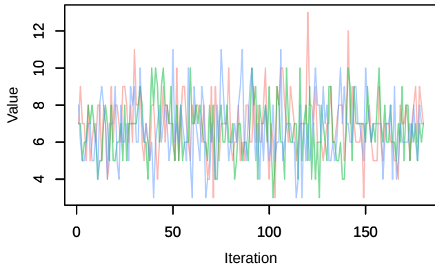
Trace – Nspecies_station[29]
