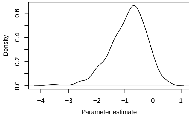
Density – beta.ranef.cont.border_dist[19]
