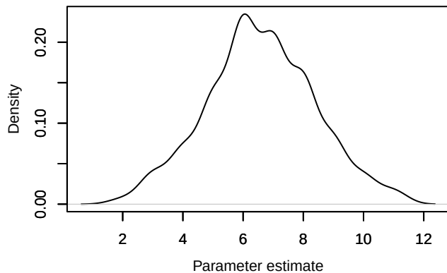
Density – Nspecies_station[26]
