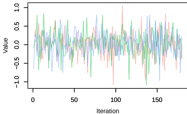
Trace – beta.ranef.cont.elev[20]
