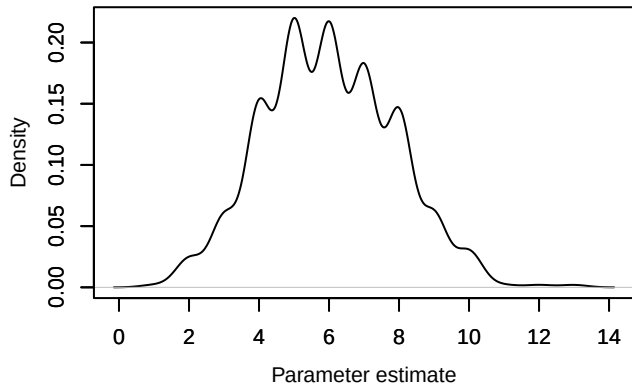
Density – Nspecies_station[8]
