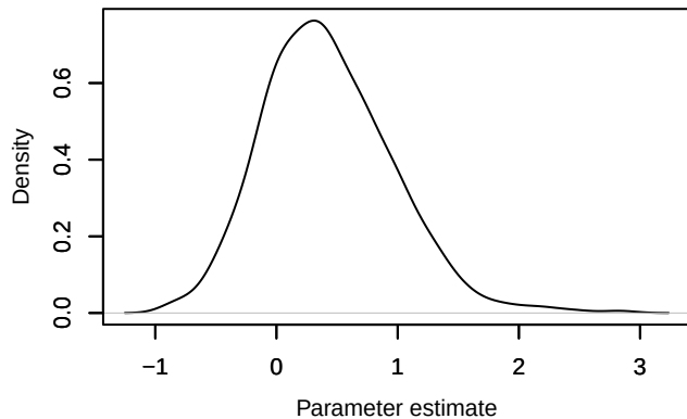
Density – beta.ranef.cont.border_dist.mean
