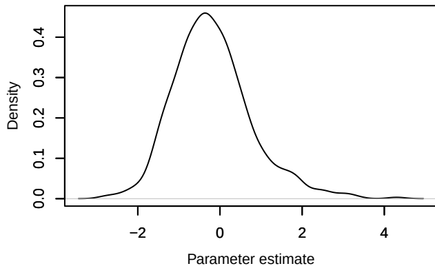
Density – beta.ranef.categ.in_AP[6,2]
