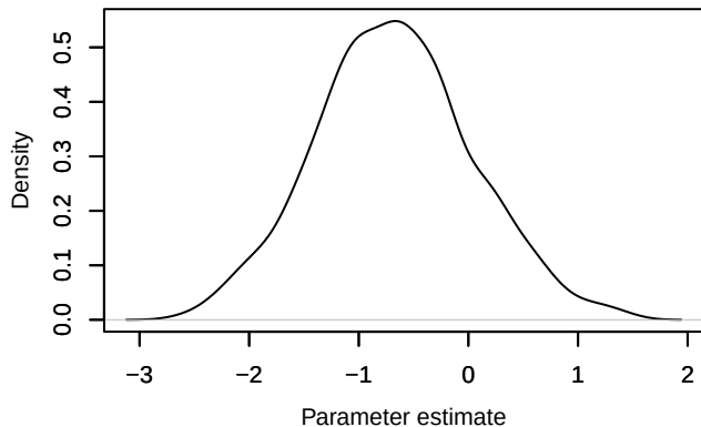
Density – beta0[2]
