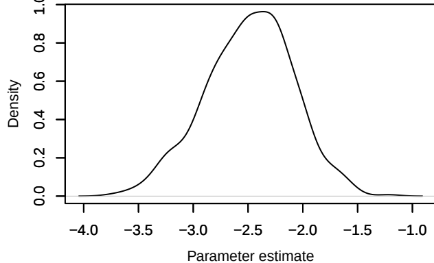
Density – alpha0[16]
