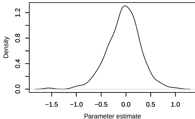
Density – beta.ranef.cont.elev[15]
