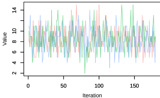
Trace – alpha.obs.fixed.cont.effort
