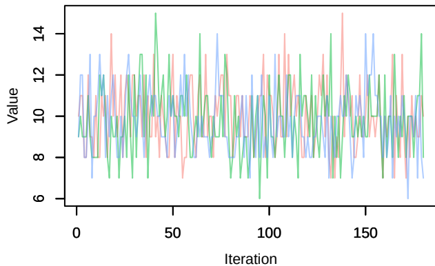
Trace – Nspecies_station[25]
