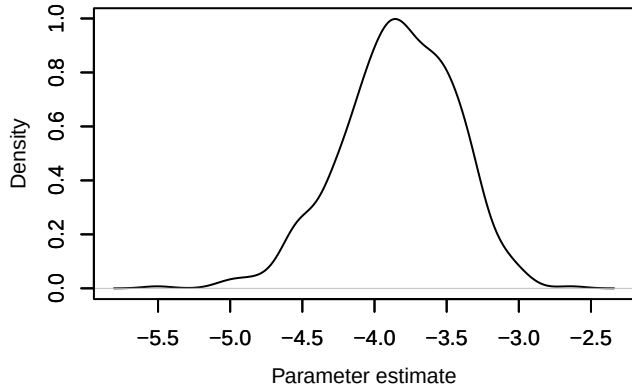
Density – alpha0[18]
