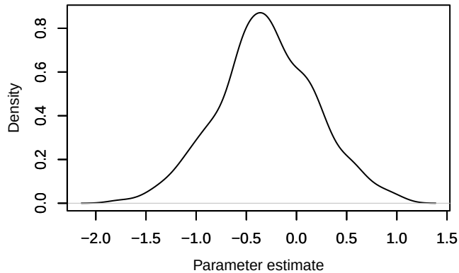
Density – beta.ranef.cont.border_dist[19]
