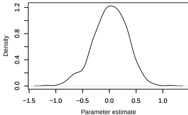
Density – beta.ranef.cont.elev[15]
