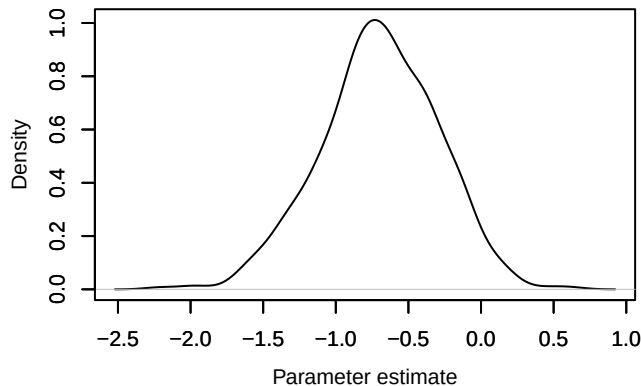
Density – beta.ranef.cont.border_dist[4]
