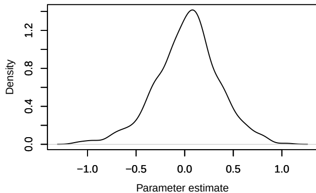
Density – beta.ranef.cont.elev[20]
