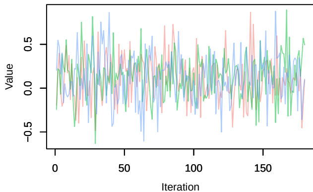
Trace – beta.ranef.cont.elev[21]
