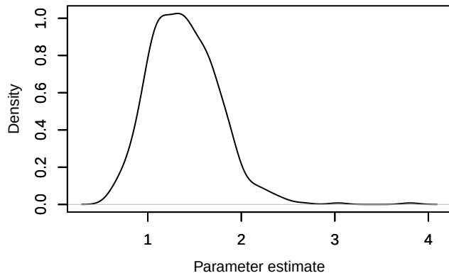
Density – beta0.sigma
