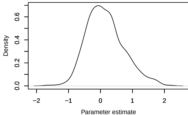
Density – beta.ranef.cont.border_dist[12]
