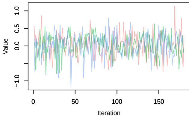
Trace – beta.ranef.cont.elev[15]
