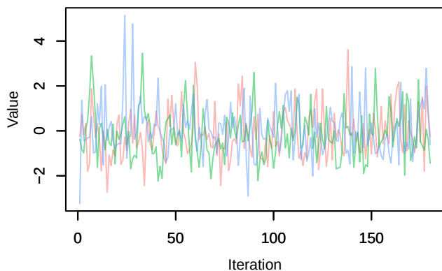
Trace – beta.ranef.categ.in_AP[13,2]
