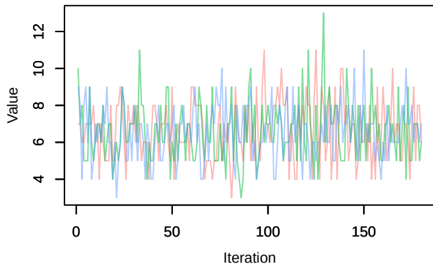
Trace – Nspecies_station[38]
