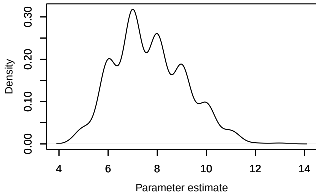
Density – Nspecies_station[17]
