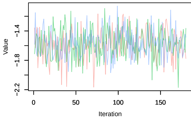
Trace – alpha0[1]
