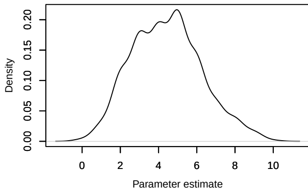
Density – Nspecies_station[31]
