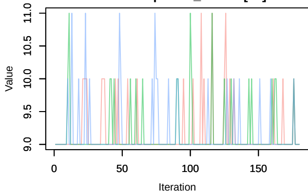
Trace – Nspecies_station[16]
