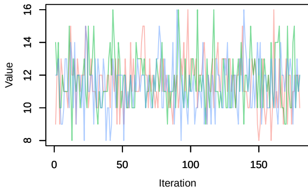
Trace – Nspecies_station[14]
