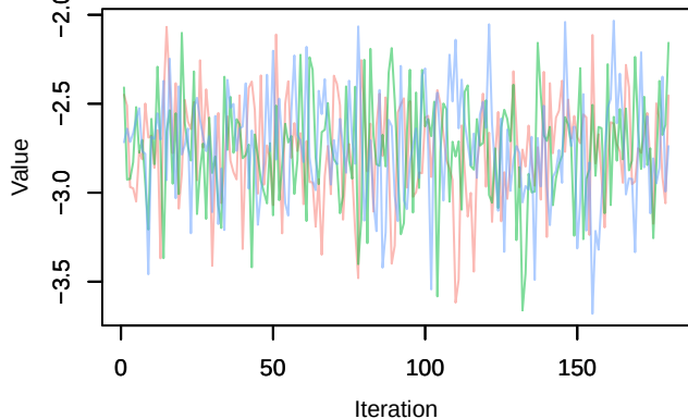
Trace – alpha0[19]
