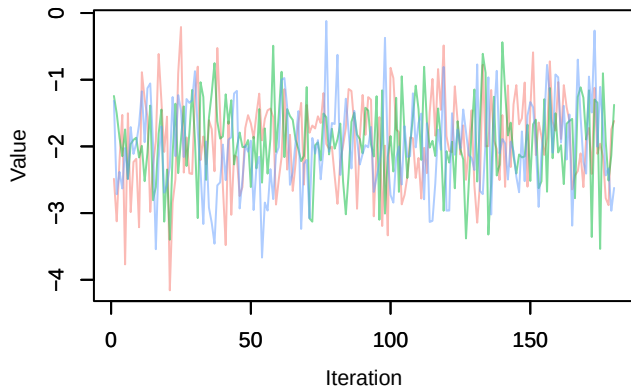
Trace – beta0[4]
