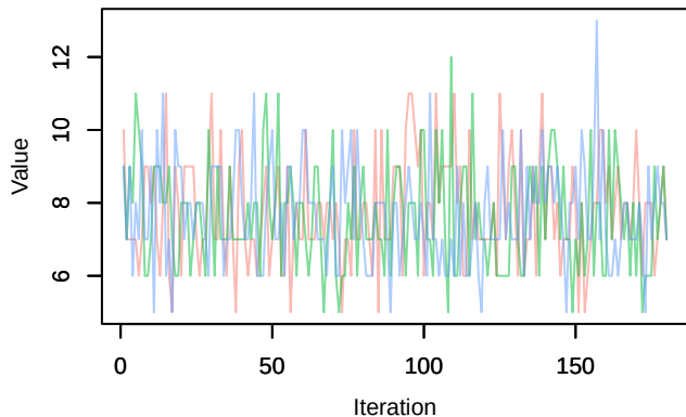
Trace – Nspecies_station[17]
