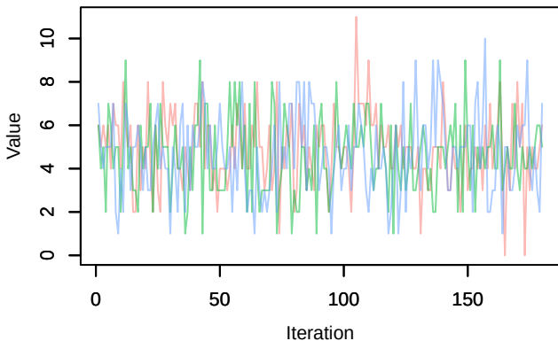
Trace – Nspecies_station[4]
