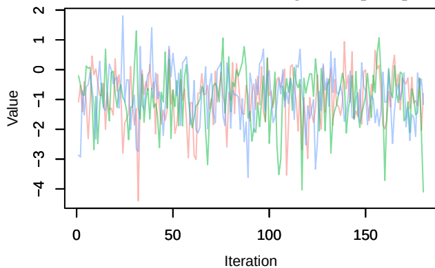
Trace – beta.ranef.category.in_AP.mean[1]
