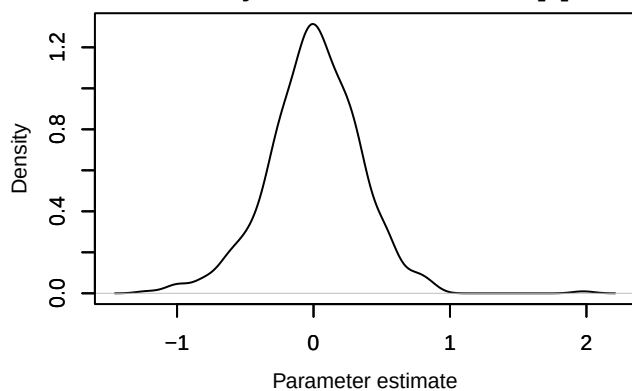
Density – beta.ranef.cont.elev[8]
