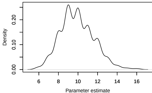
Density – Nspecies_station[2]
