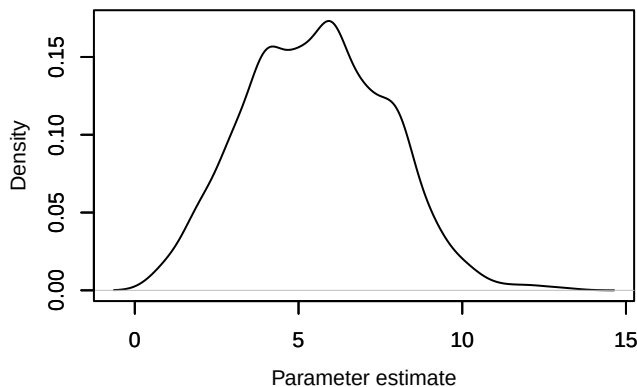
Density – Nspecies_station[10]
