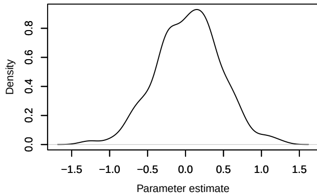
Density – beta.ranef.cont.border_dist[22]
