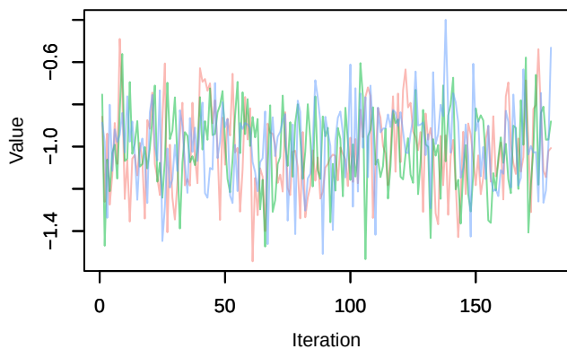
Trace – alpha0[4]
