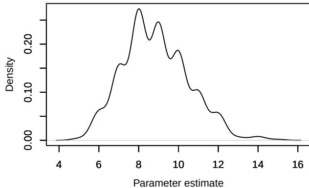
Density – Nspecies_station[23]
