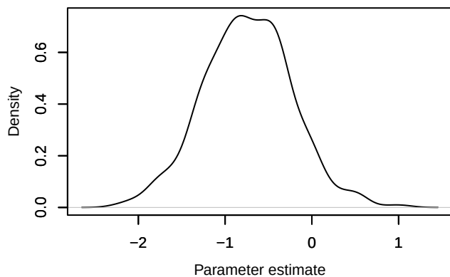
Density – beta.ranef.category.in_AP.mean[2]
