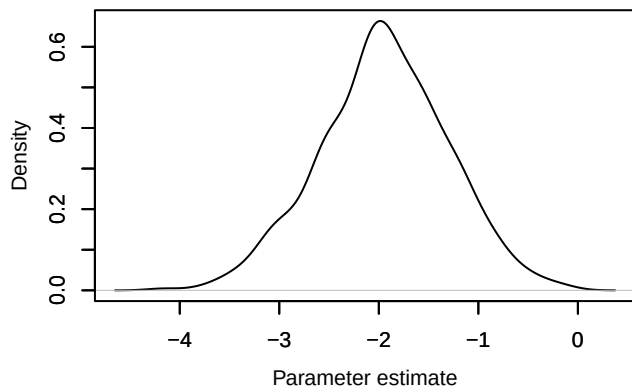
Density – beta0[4]
