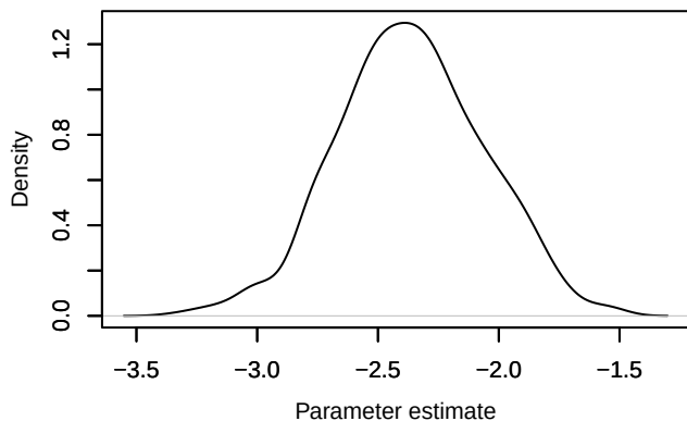
Density – alpha0.mean
