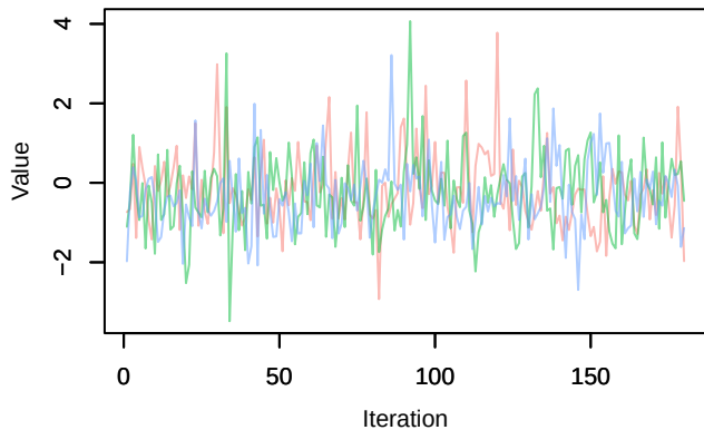
Trace – beta0[19]
