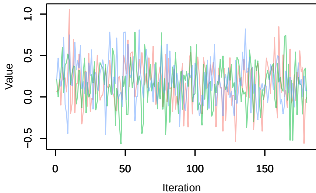
Trace – beta.ranef.cont.elev[2]
