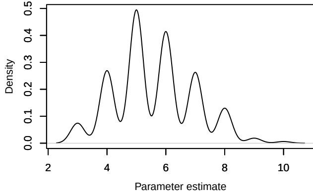
Density – Nspecies_station[38]
