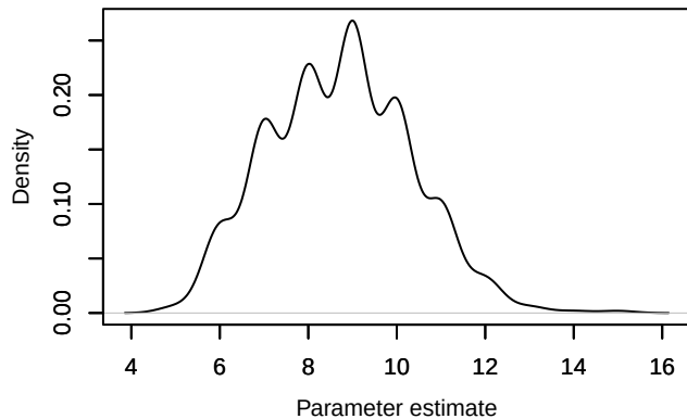
Density – Nspecies_station[22]
