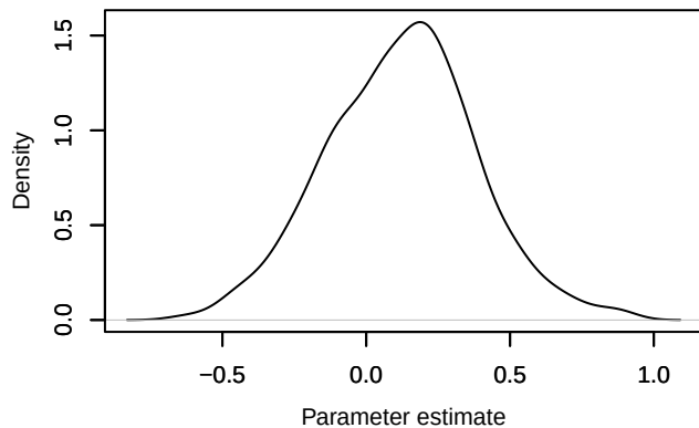
Density – beta.ranef.cont.elev[21]
