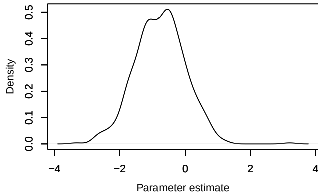
Density – beta.ranef.categ.in_AP[3,2]
