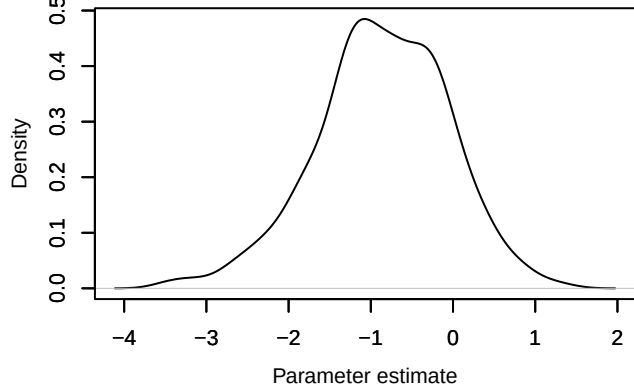
Density – beta.ranef.categ.in_AP[4,2]
