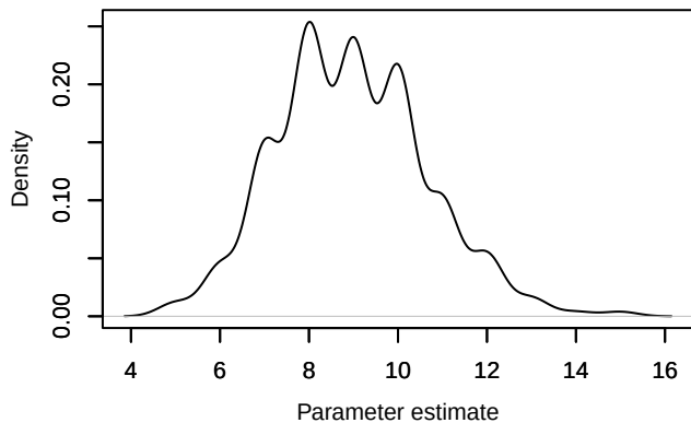
Density – Nspecies_station[17]
