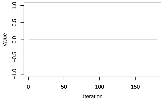
Trace – beta.ranef.categ.in_AP[18,1]
