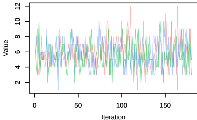
Trace – Nspecies_station[10]
