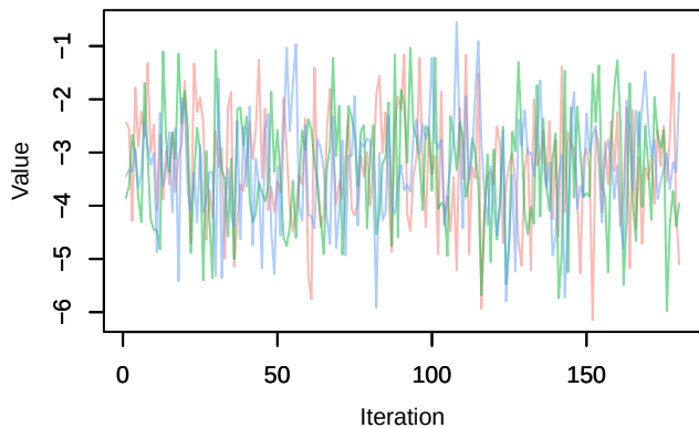
Trace – alpha0[21]
