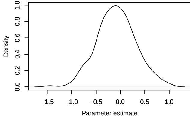
Density – beta.ranef.cont.border_dist[4]
