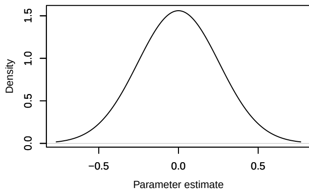
Density – beta.ranef.categ.in_AP[6,1]
