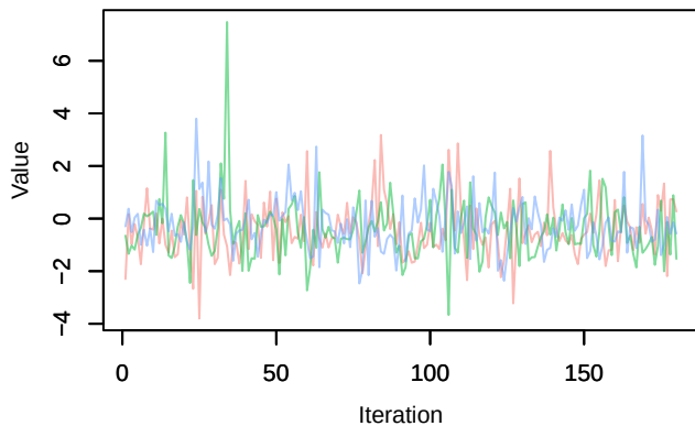
Trace – beta.ranef.categ.in_AP[15,2]
