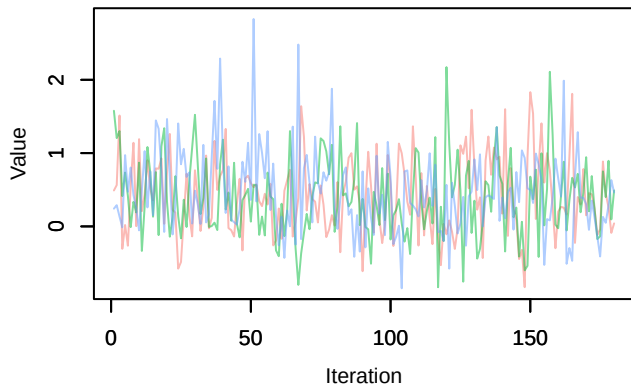
Trace – beta.ranef.cont.border_dist.mean
