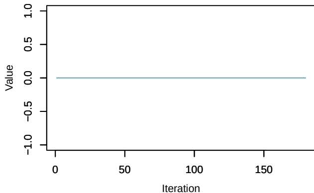
Trace – beta.ranef.categ.in_AP[9,1]
