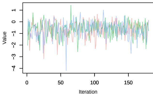
Trace – beta.ranef.cont.border_dist[7]
