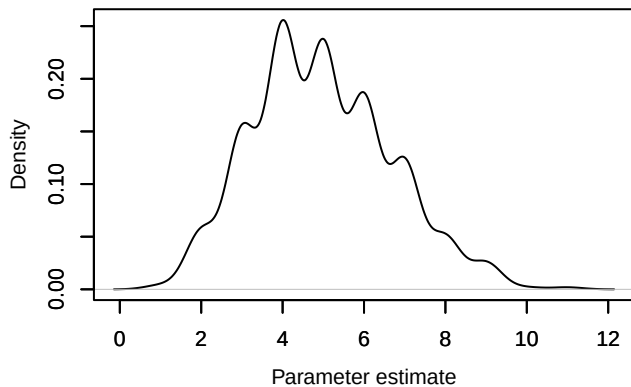
Density – Nspecies_station[47]
