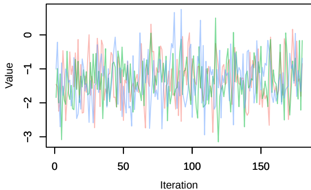
Trace – beta0[22]
