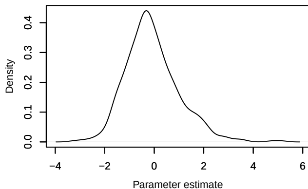
Density – beta.ranef.categ.in_AP[13,2]
