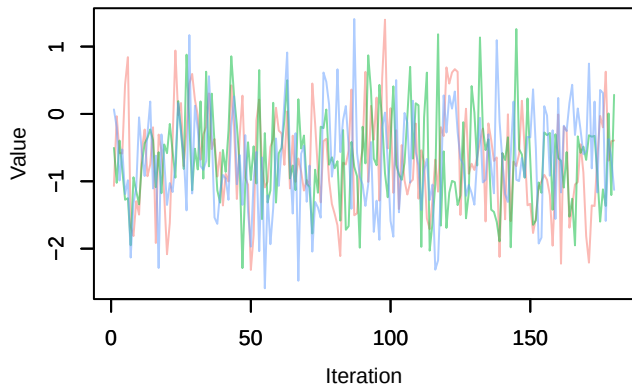
Trace – beta0[2]
