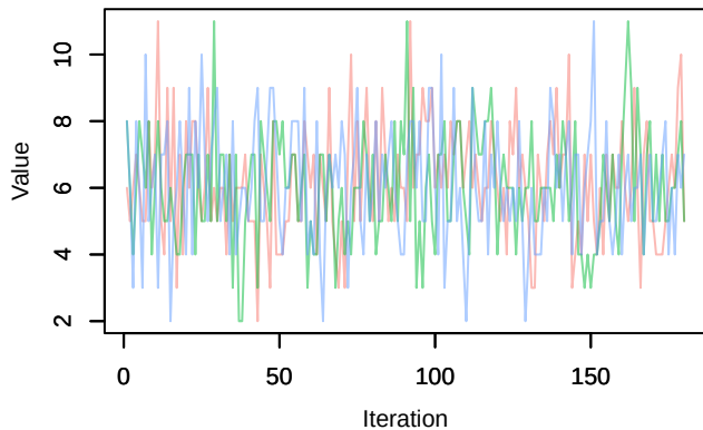
Trace – Nspecies_station[28]
