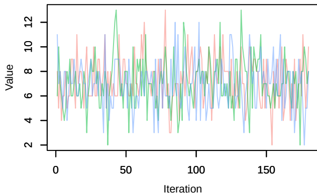
Trace – Nspecies_station[32]
