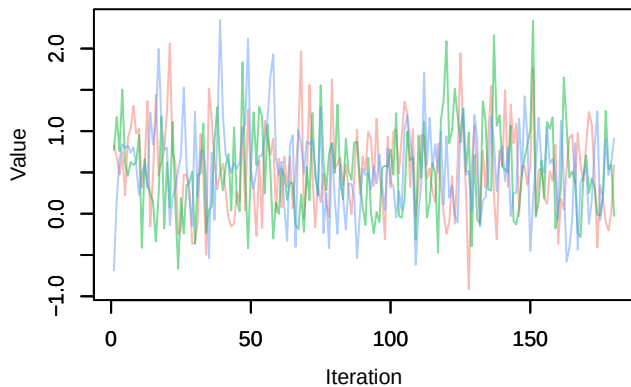
Trace – beta.ranef.cont.border_dist[10]
