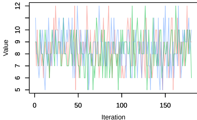
Trace – Nspecies_station[8]
