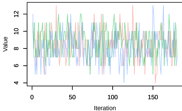
Trace – Nspecies_station[37]
