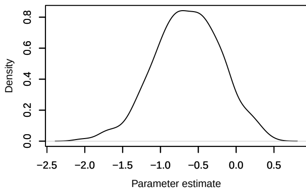
Density – beta.ranef.cont.border_dist[6]
