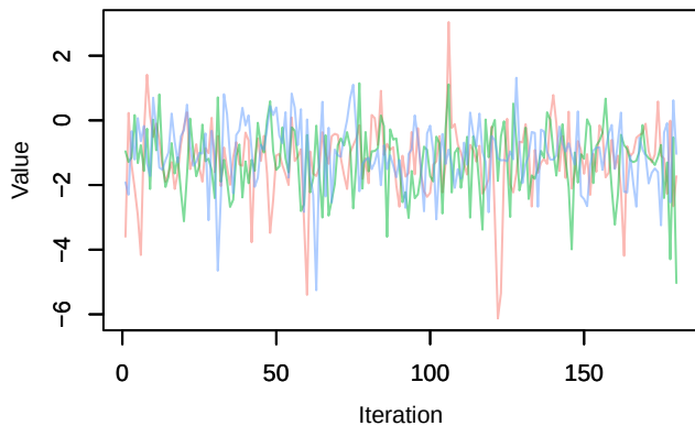
Trace – beta.ranef.categ.in_AP[18,2]
