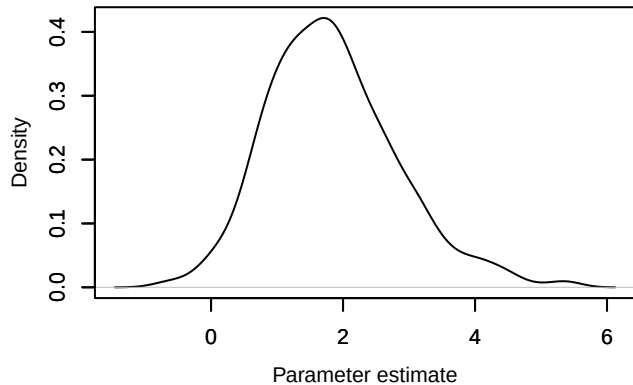
Density – beta0[8]
