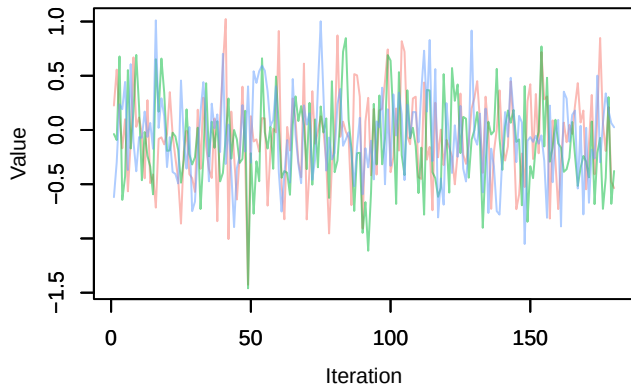
Trace – beta.ranef.cont.border_dist[4]
