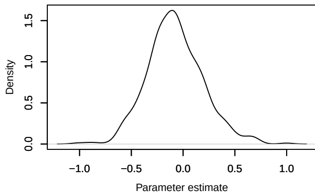
Density – beta.ranef.cont.border_dist.sigma
