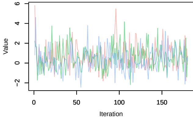
Trace – beta0[14]
