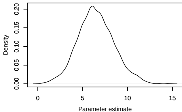
Density – Nspecies_station[62]
