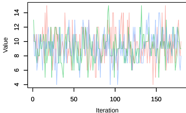
Trace – Nspecies_station[41]
