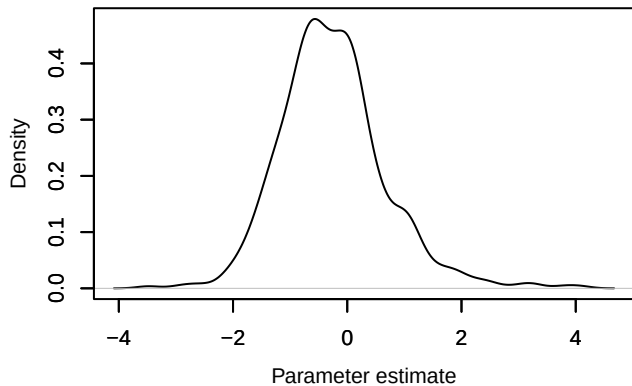
Density – beta0[19]
