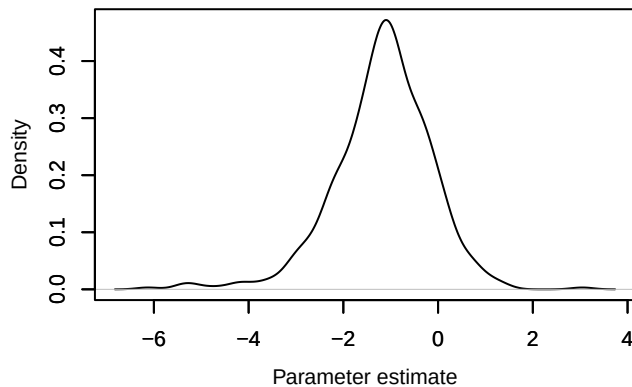
Density – beta.ranef.categ.in_AP[18,2]
