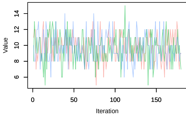
Trace – Nspecies_station[49]
