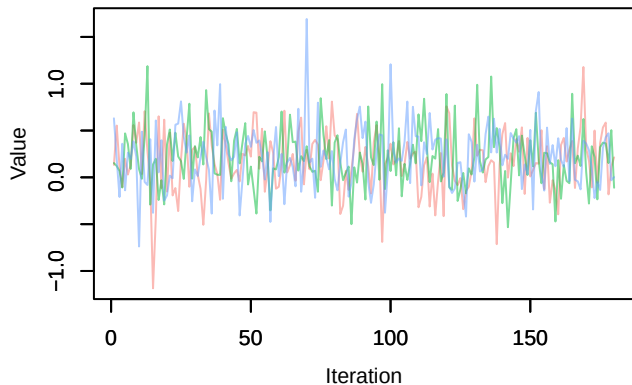
Trace – beta.ranef.cont.elev[12]
