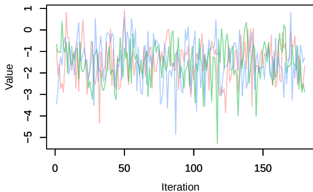
Trace – beta.ranef.categ.in_AP[1,2]
