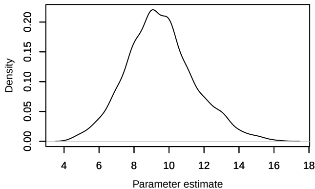
Density – Nspecies_station[5]
