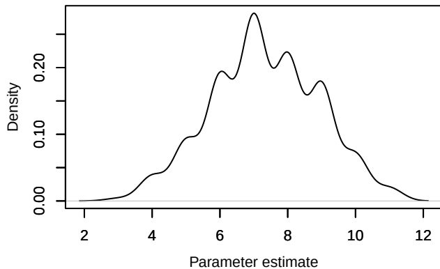
Density – Nspecies_station[40]
