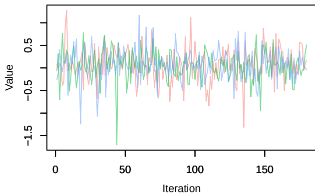
Trace – beta.ranef.cont.elev[17]
