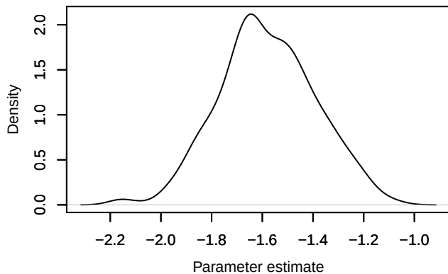
Density – alpha0[1]
