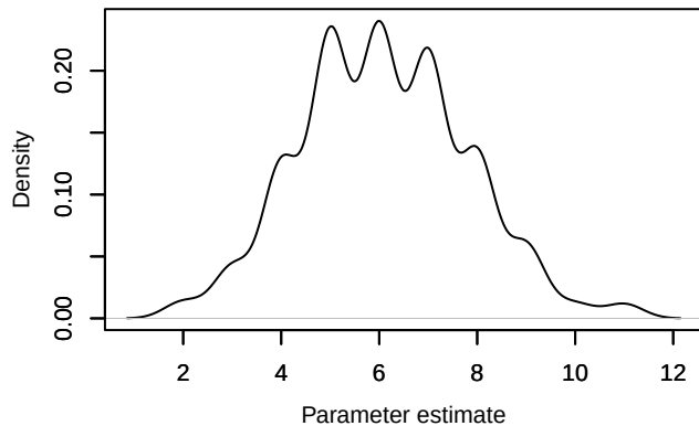
Density – Nspecies_station[28]
