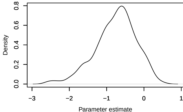
Density – beta.ranef.cont.border_dist[5]
