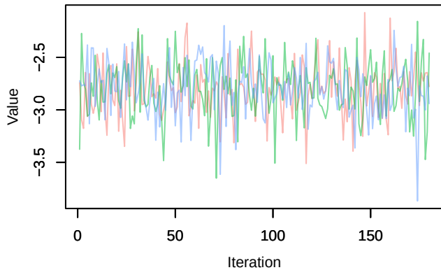
Trace – alpha0[16]
