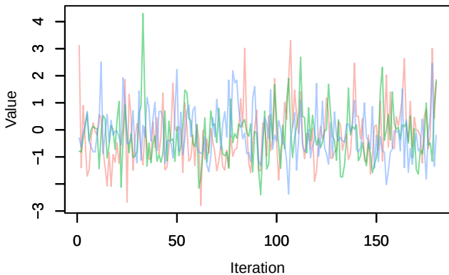
Trace – beta.ranef.categ.in_AP[6,2]
