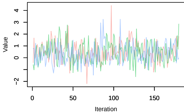
Trace – beta0[16]
