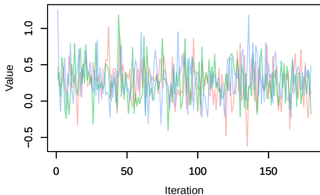
Trace – beta.ranef.cont.elev[3]
