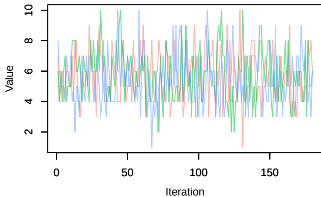
Trace – Nspecies_station[55]
