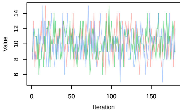
Trace – Nspecies_station[53]
