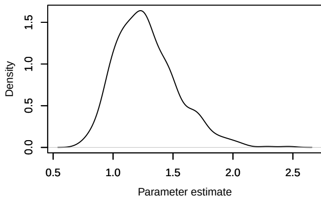
Density – alpha0.sigma
