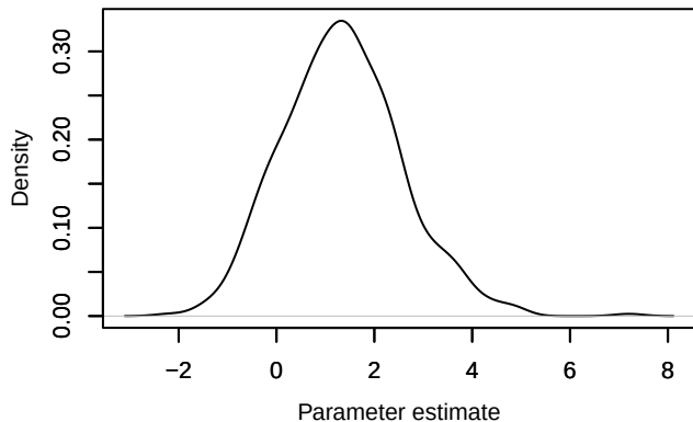
Density – beta0[14]
