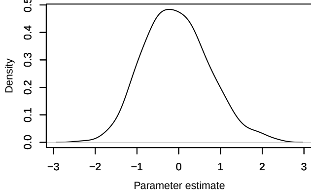
Density – beta.ranef.categ.in_AP[7,2]
