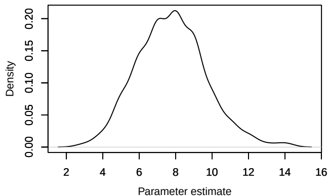
Density – Nspecies_station[56]
