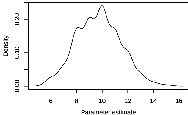
Density – Nspecies_station[50]
