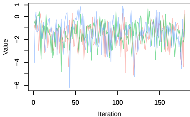
Trace – beta.ranef.categ.in_AP[12,2]
