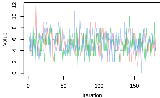
Trace – Nspecies_station[59]
