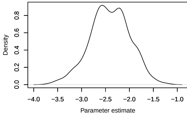
Density – alpha0[22]
