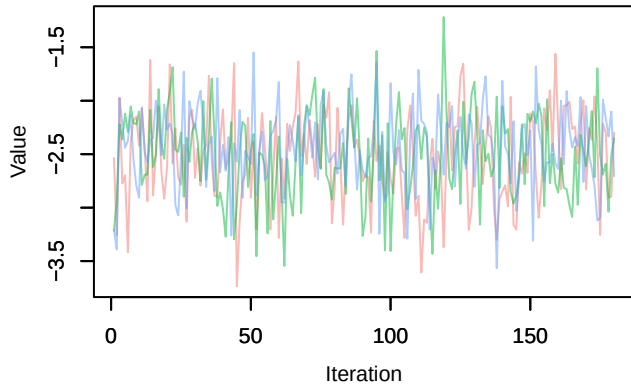
Trace – alpha0[16]
