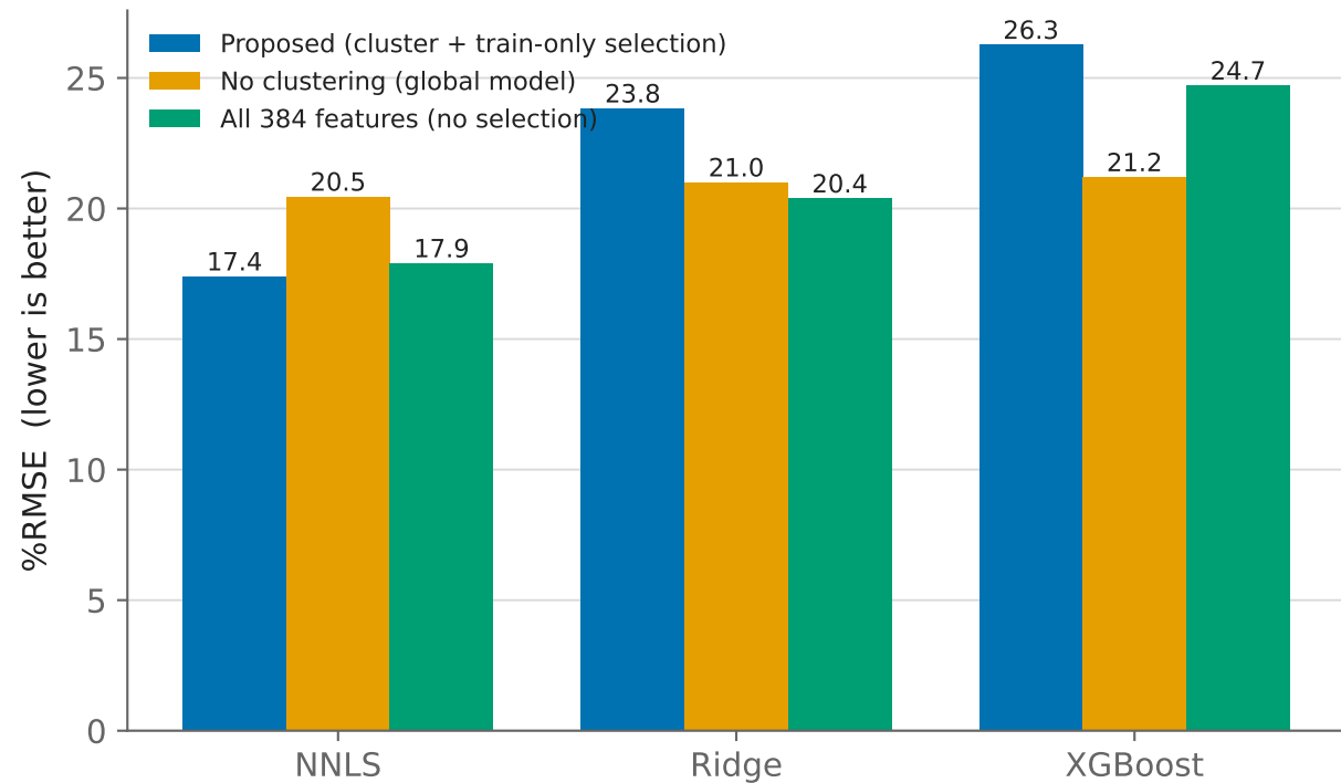
Germany ablation (DINOv2) — leak-free
