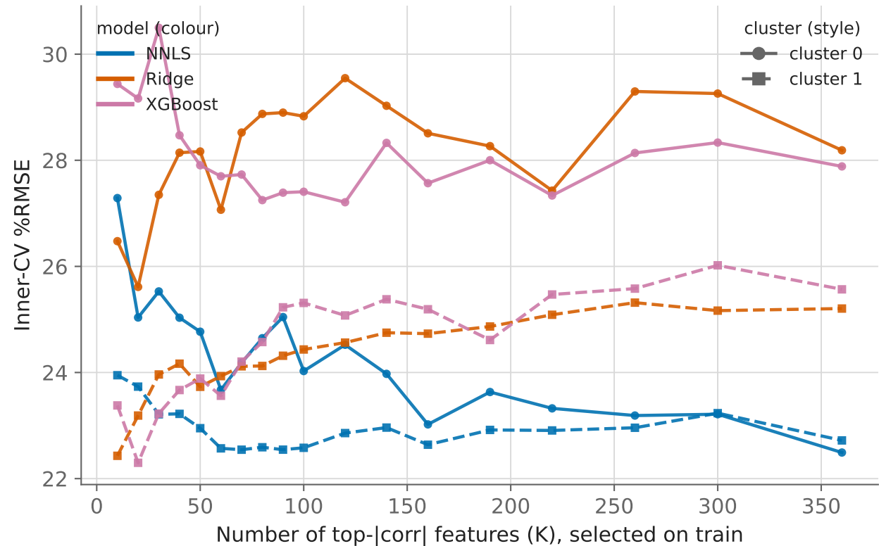
Germany DINO — train-only CV vs. feature count
