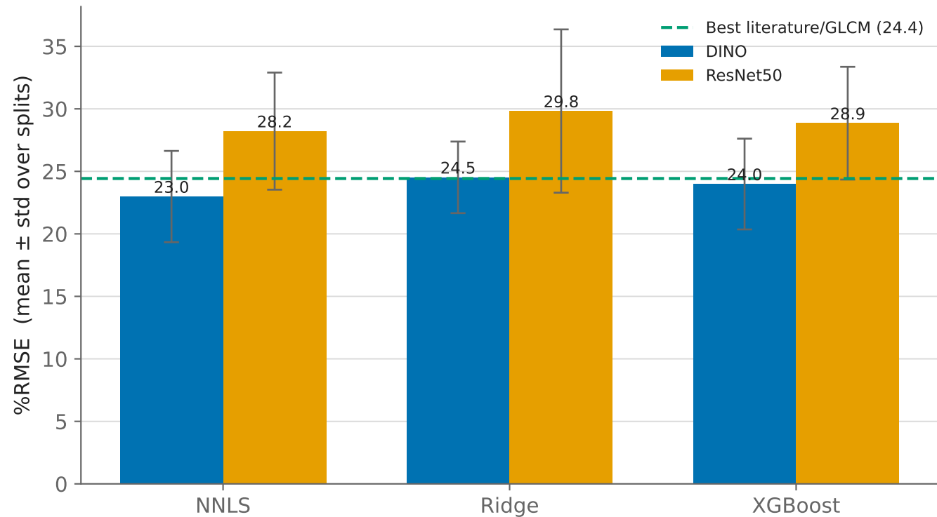
Germany robustness — proposed pipeline over 20 stratified 85/15 splits
