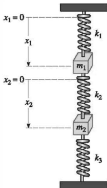
FIGURE 4.6.4 Coupled springs in Problem 14
