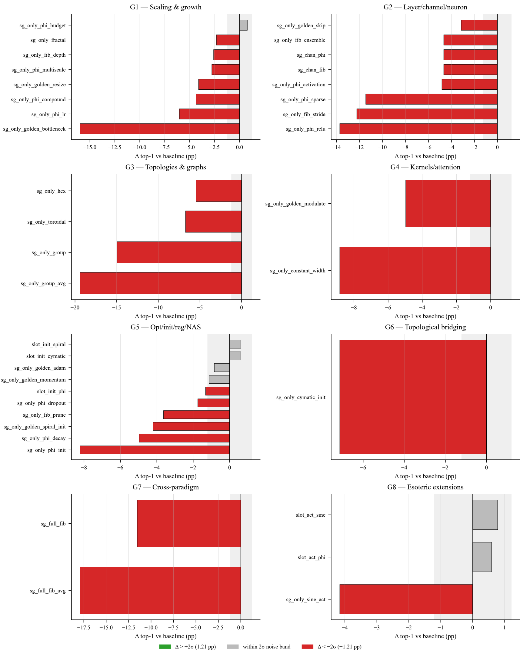
Figure 2 — CIFAR-10 12-ep ablation per group ( \Delta top-1 vs baseline_resnet20 seed-0)
