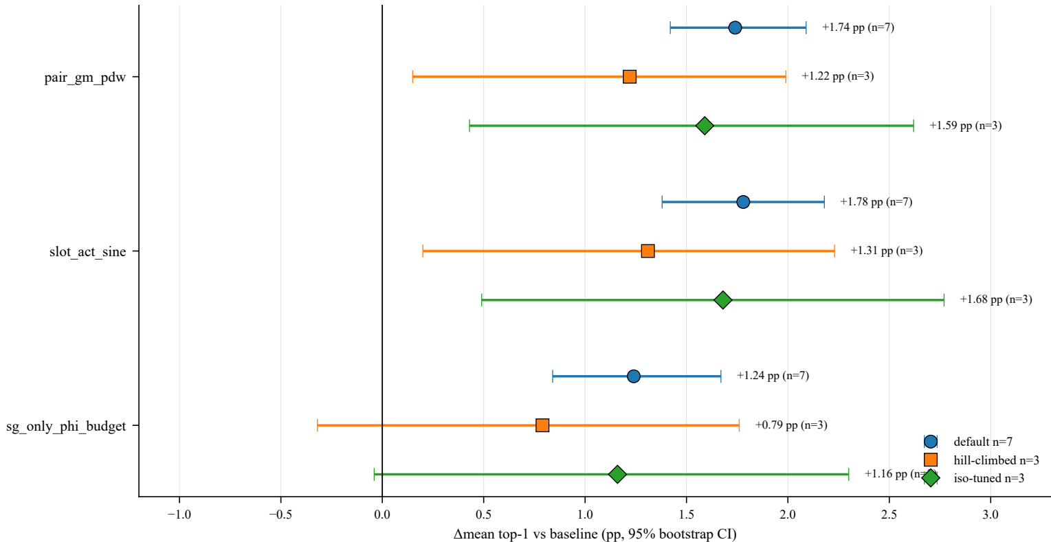
Figure 3 — Three robustness regimes for Phase-8 winners (CIFAR-100, 30 epochs)
